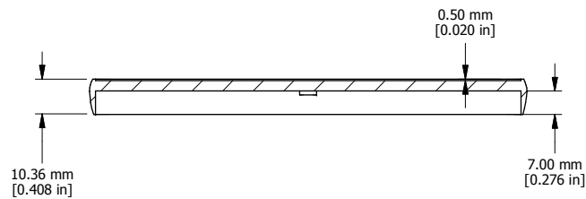
CLOSED BEZEL
