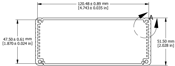
EXTRUSION
