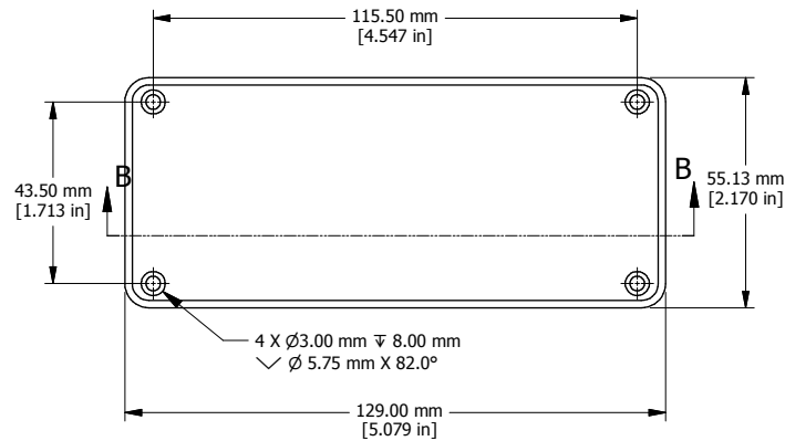
CLOSED BEZEL
