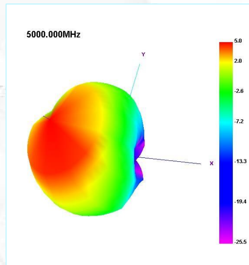
5000MHz Radiation Pattern
