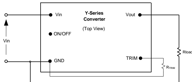
Fig. D: Configuration for programming output voltage.
