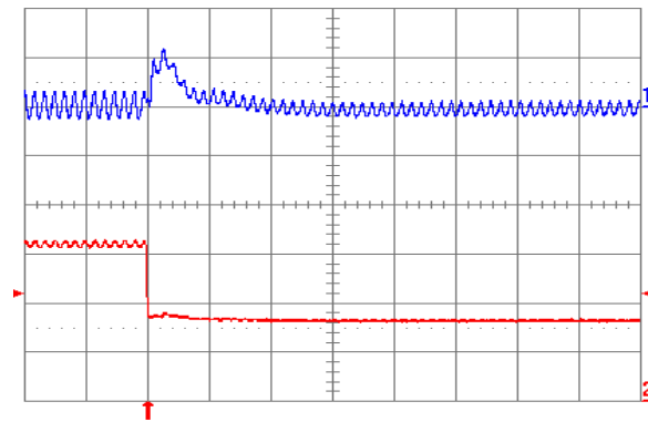
Fig. 1.5V.8: Output voltage response for V_{out} = 1.5\text{ V} to negative load current step change from 5 A to 2.5 A with slew rate of -5\text{ A}/\mu\text{s} at V_{in} = 5\text{ V} . Top trace: output voltage (100 mV/div.); Bottom trace: load current (2 A/div.). C_o = 47\text{ }\mu\text{F} ceramic + 1\text{ }\mu\text{F} ceramic. Time scale: 20 \mu\text{s} /div.
