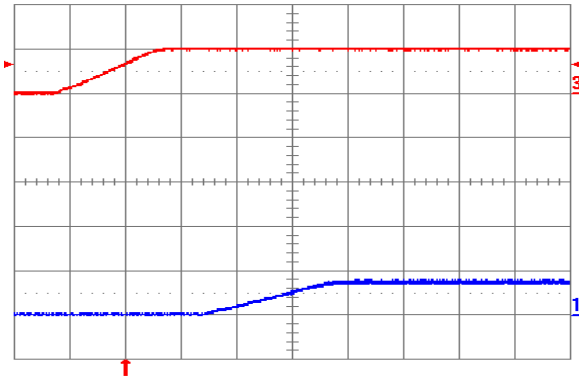
Fig. 0.7525V.4: Turn-on transient for V_{out} = 0.7525 V with application of V_{in} at full rated load current (resistive) and 47 \mu F external capacitance at V_{in} = 5 V. Top trace: V_{in} (5 V/div.); Bottom trace: output voltage (1 V/div.); Time scale: 2 ms/div.
