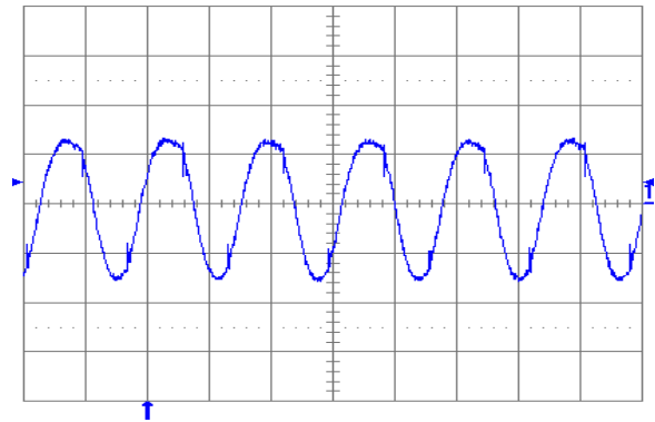
Fig. 2.5V.5: Output voltage ripple (20 mV/div.) at full rated load current into a resistive load with external capacitance 10\text{ }\mu\text{F} ceramic + 1\text{ }\mu\text{F} ceramic and V_{in} = 5\text{ V} for V_{out} = 2.5\text{ V} . Time scale: 2 \mu\text{s} /div.
