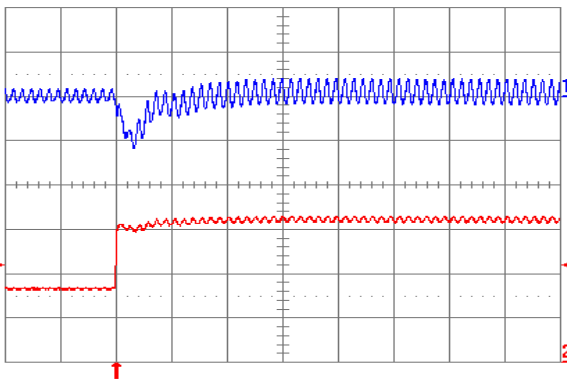
Fig. 1.5V.7: Output voltage response for V_{out} = 1.5\text{ V} to positive load current step change from 2.5 A to 5 A with slew rate of 5\text{ A}/\mu\text{s} at V_{in} = 5\text{ V} . Top trace: output voltage (100 mV/div.); Bottom trace: load current (2 A/div.). C_o = 47\text{ }\mu\text{F} ceramic + 1\text{ }\mu\text{F} ceramic. Time scale: 20 \mu\text{s} /div.
