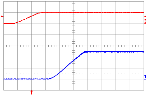
Fig. 2.5V.4: Turn-on transient for V_{out} = 2.5\text{ V} with application of V_{in} at full rated load current (resistive) and 47\text{ }\mu\text{F} external capacitance at V_{in} = 5\text{ V} . Top trace: V_{in} (5 V/div.); Bottom trace: output voltage (1V/div.); Time scale: 2 ms/div.
