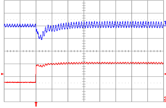
Fig. 1.2V.6: Output voltage response for V_{out} = 1.2\text{ V} to positive load current step change from 2.5 A to 5 A with slew rate of 5\text{ A}/\mu\text{s} at V_{in} = 5\text{ V} . Top trace: output voltage (100 mV/div.); Bottom trace: load current (2 A/div.). C_o = 47\text{ }\mu\text{F} ceramic + 1\text{ }\mu\text{F} ceramic. Time scale: 20\text{ }\mu\text{s}/\text{div} .
