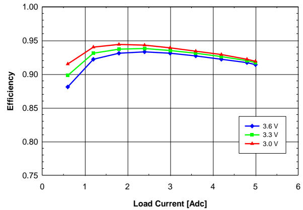
Fig. 2.0V.4: Efficiency vs. load current and input voltage for V_{out} = 2.0\text{ V} converter mounted horizontally with air flowing from pin 5 to pin 1 at a rate of 200 LFM (1 m/s) and T_a = 25\text{ }^{\circ}\text{C} .
