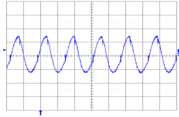
Fig. 1.5V.6: Output voltage ripple (20 mV/div.) at full rated load current into a resistive load with external capacitance 10\text{ }\mu\text{F} ceramic + 1\text{ }\mu\text{F} ceramic and V_{in} = 5\text{ V} for V_{out} = 1.5\text{ V} . Time scale: 2 \mu\text{s} /div.
