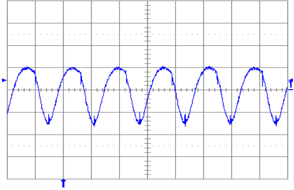
Fig. 3.3V.6: Output voltage ripple ( 20\text{ mV/div.} ) at full rated load current into a resistive load with external capacitance 10\text{ }\mu\text{F} ceramic + 1\text{ }\mu\text{F} ceramic and V_{in} = 5\text{ V} for V_{out} = 3.3\text{ V} . Time scale: 2\text{ }\mu\text{s/div.}
