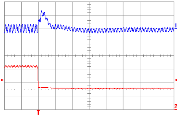
Fig. 2.5V.8: Output voltage response for V_{out} = 2.5\text{ V} to negative load current step change from 5 A to 2.5 A with slew rate of -5\text{ A}/\mu\text{s} at V_{in} = 5\text{ V} . Top trace: output voltage (100 mV/div.); Bottom trace: load current (2 A/div.). C_o = 47\text{ }\mu\text{F} ceramic + 1\text{ }\mu\text{F} ceramic. Time scale: 20 \mu\text{s} /div.
