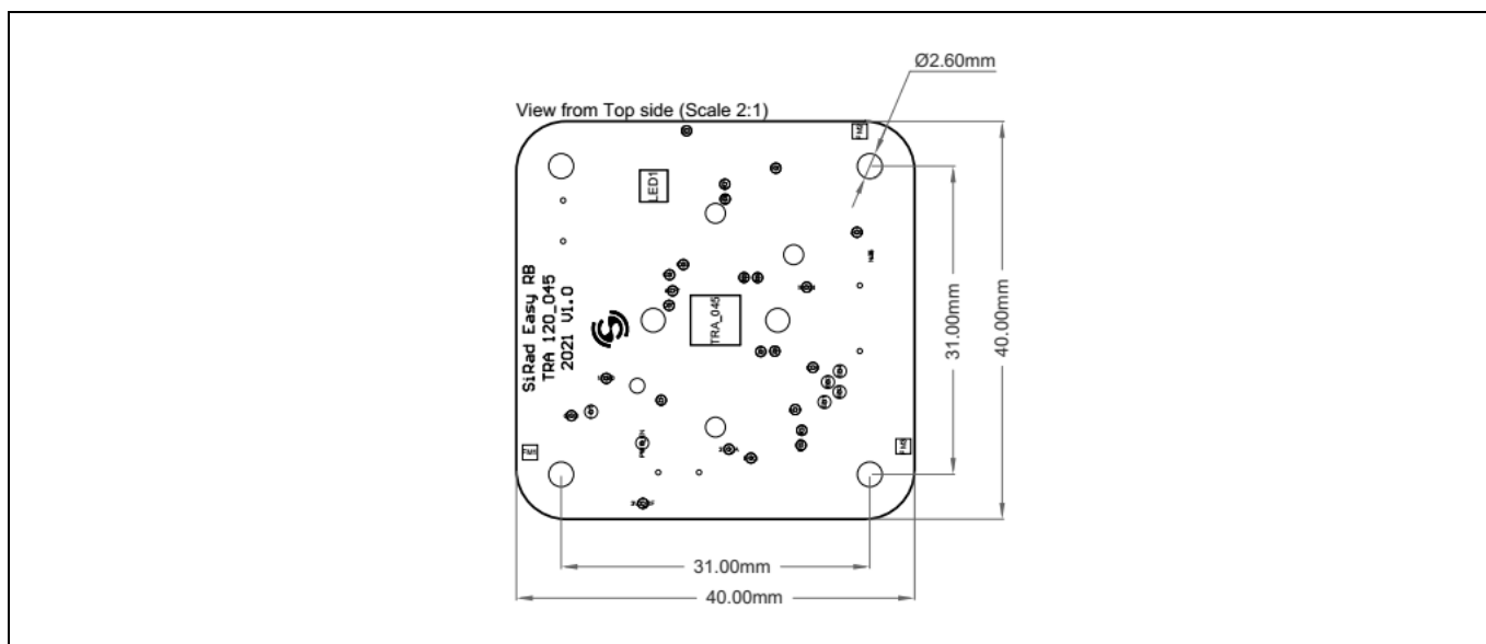
Figure 1 Mechanical Drawing
