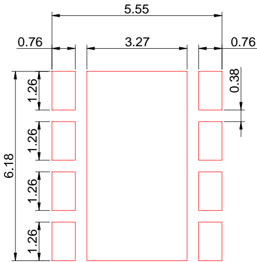
Recommended Solder Pad
