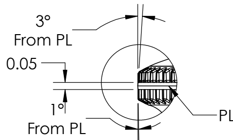
DETAIL C SCALE 1.5 : 1
