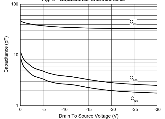
Fig. 6 - Capacitance Characteristics
