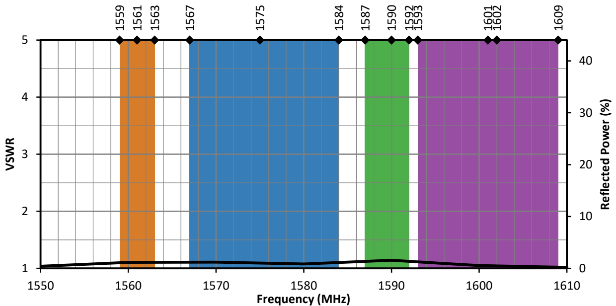
Figure 1. ANT-GNCP-CA188L165 VSWR with Frequency Band Highlights
