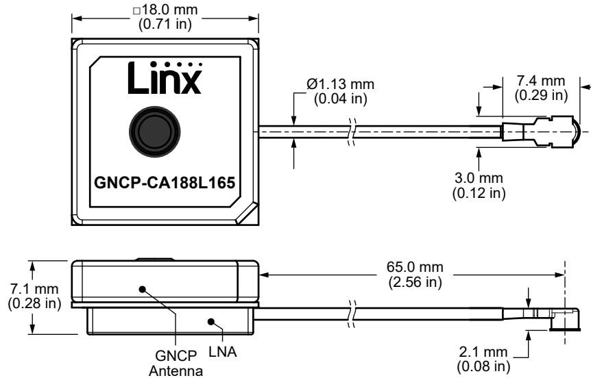
Figure 6. ANT-GNCP-CA188L165 Antenna Dimensions
