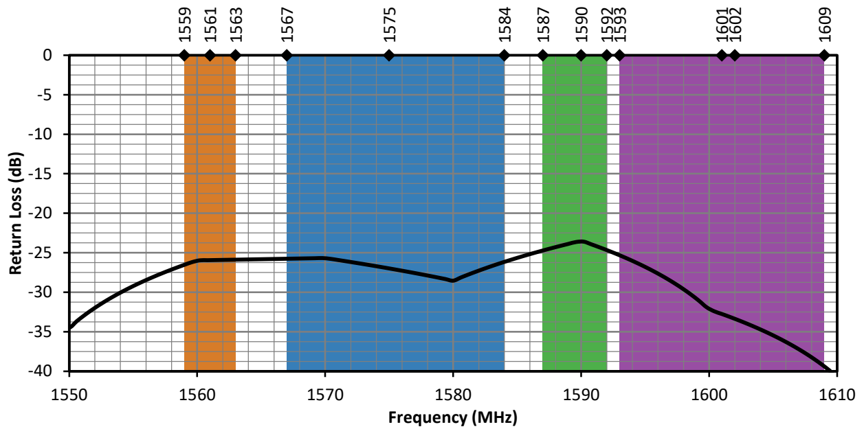
Figure 2. ANT-GNCP-CA188L165 Return Loss with Frequency Band Highlights
