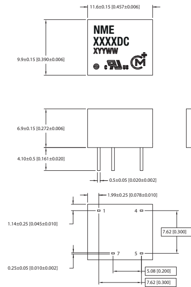
DIP Package
