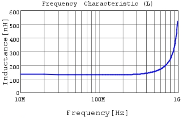
LQG15WZR13G02 L
