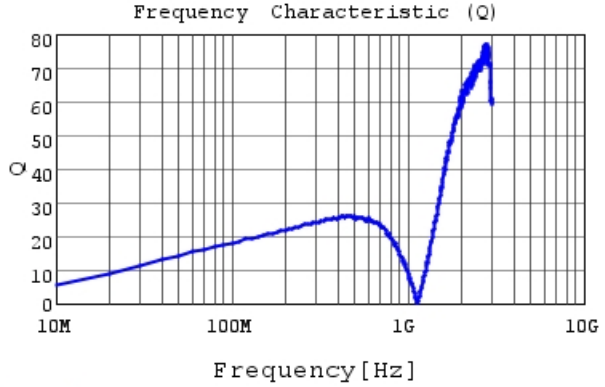
LQG15WZR13G02 Q
