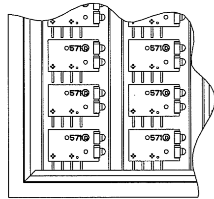
PACKAGING DETAIL
