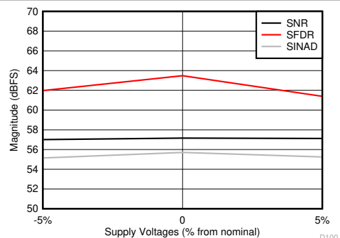
All supplies changed together, high power mode Figure 8-60. SNR, SFDR and SINAD vs Supply Voltage
