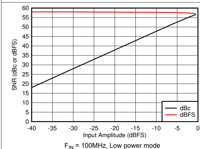
Figure 8-35. SNR vs A_{IN}
