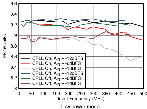
Figure 8-57. ENOB vs A_{IN} and C-PLL
