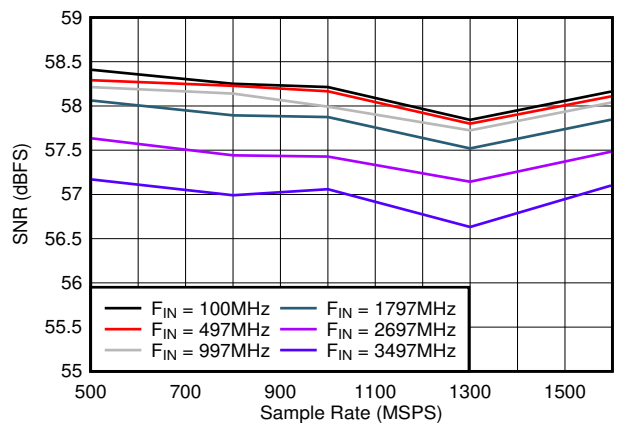
Figure 8-24. SNR vs Sample Rate
