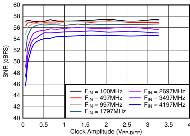
Figure 8-37. SNR vs A_{CLK}
