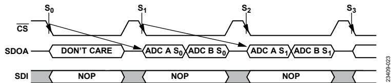
Figure 41. Read Conversion Results for 1-Wire Mode
