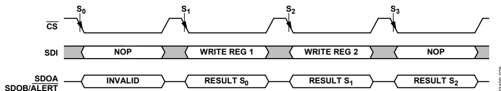
Figure 44. Register Write
