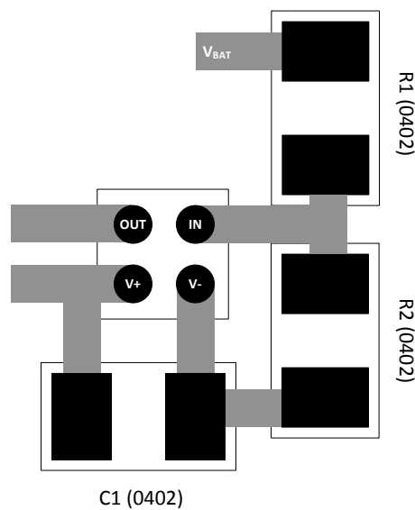
Figure 11-1. Layout Example
