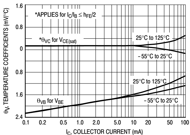
Figure 9. Temperature Coefficients
