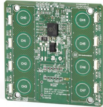
Figure 1. NCN5140TSCGEVB Switch Application Board Touch Version
