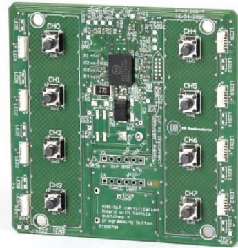
Figure 2. NCN5140BSCGEVB Switch Application Board Tactile Version
