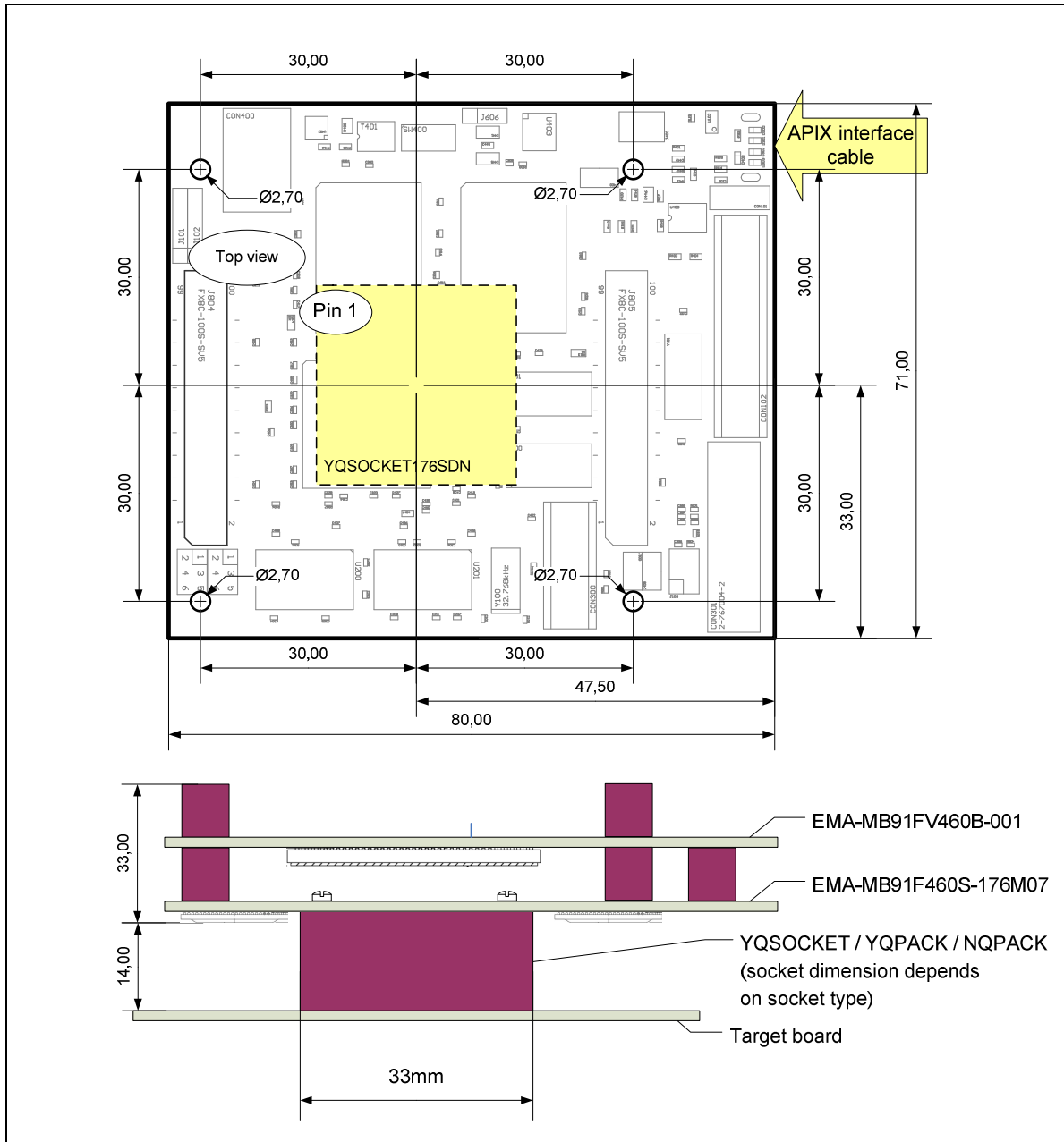
Figure 5-1: Mechanical Dimensions
