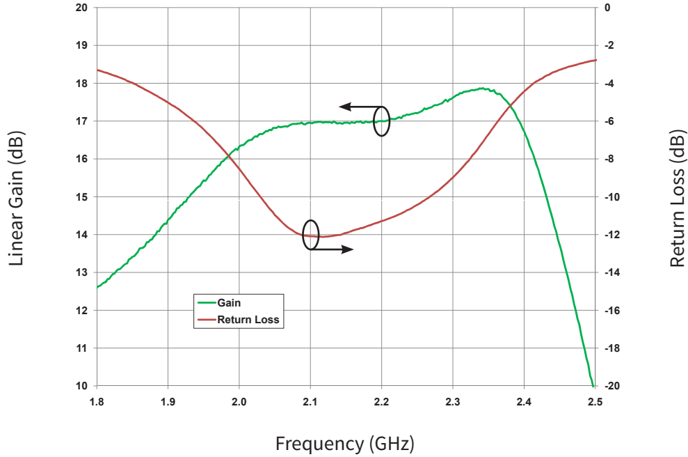
Typical Small Signal Gain and Return Loss vs Frequency of the CGH21240F measured in CGH21240F-AMP Amplifier Circuit V_{DS} = 28\text{ V}, I_{DS} = 1.0\text{ A}
