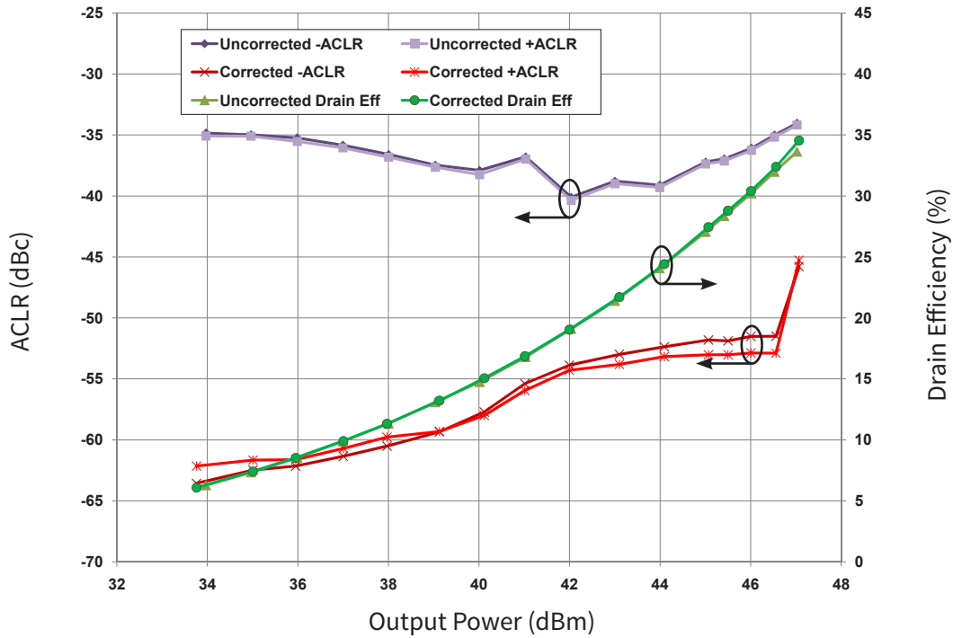
WCDMA Characteristics with and without DPD Correction ACLR and Drain Efficiency vs Output Power of the CGH21240F measured in CGH21240F-AMP Amplifier Circuit V_{DS} = 28\text{ V} , I_{DS} = 1.0\text{ A} , Frequency = 2.14 GHz
