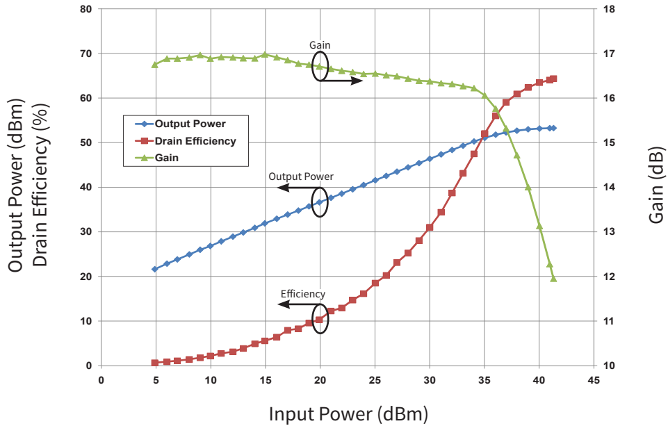
Typical Pulsed Output Power, Drain Efficiency, and Gain vs Input Power of the CGH21240F measured in CGH21240F-AMP Amplifier Circuit V_{DS} = 28\text{ V} , I_{DS} = 1.0\text{ A} , Freq = 2.14 GHz, Pulse Width = 40 \mu\text{S} , Duty Cycle = 5%
