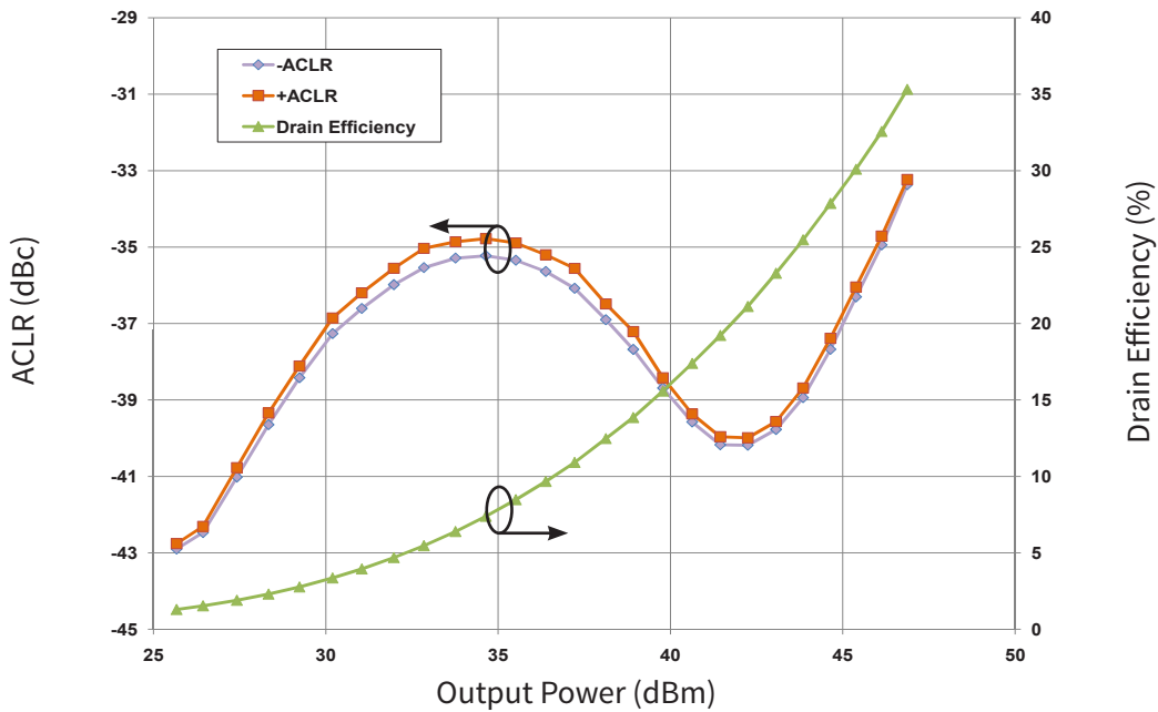
Typical WCDMA Characteristics ACLR and Drain Efficiency vs Output Power of the CGH21240F measured in CGH21240F-AMP Amplifier Circuit. 3GPP Test Model 1, 64 DPCCH 67% Clipping, 8.81 dB PAR @ 0.01% V_{DS} = 28\text{ V}, I_{DS} = 1.0\text{ A}, \text{Frequency} = 2.14\text{ GHz}
