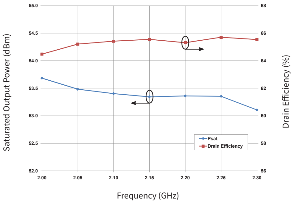
Typical Pulsed Saturated Power and Drain Efficiency vs Frequency of the CGH21240F measured in CGH21240F-AMP Amplifier Circuit. V_{DS} = 28\text{ V} , I_{DS} = 1.0\text{ A} , P_{SAT} = 20\text{ mA } I_{GS} Peak, Pulse Width = 40 \mu\text{S} , Duty Cycle = 5%
