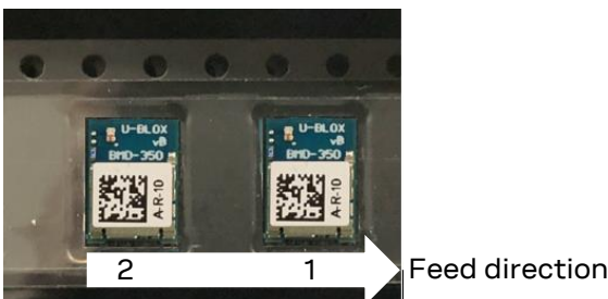
Figure 15: Carrier tape orientation
