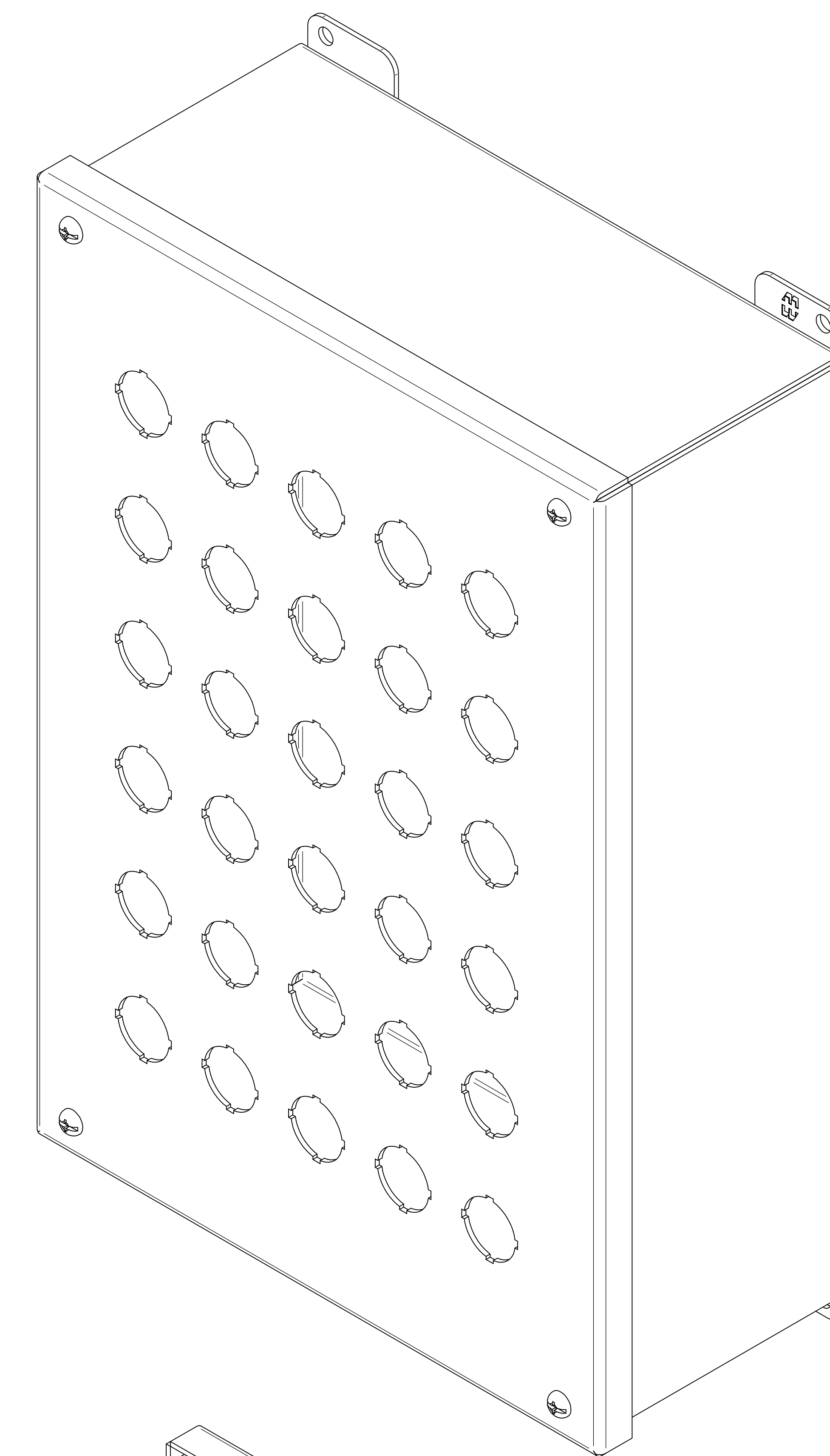
ISOMETRIC VIEWS
