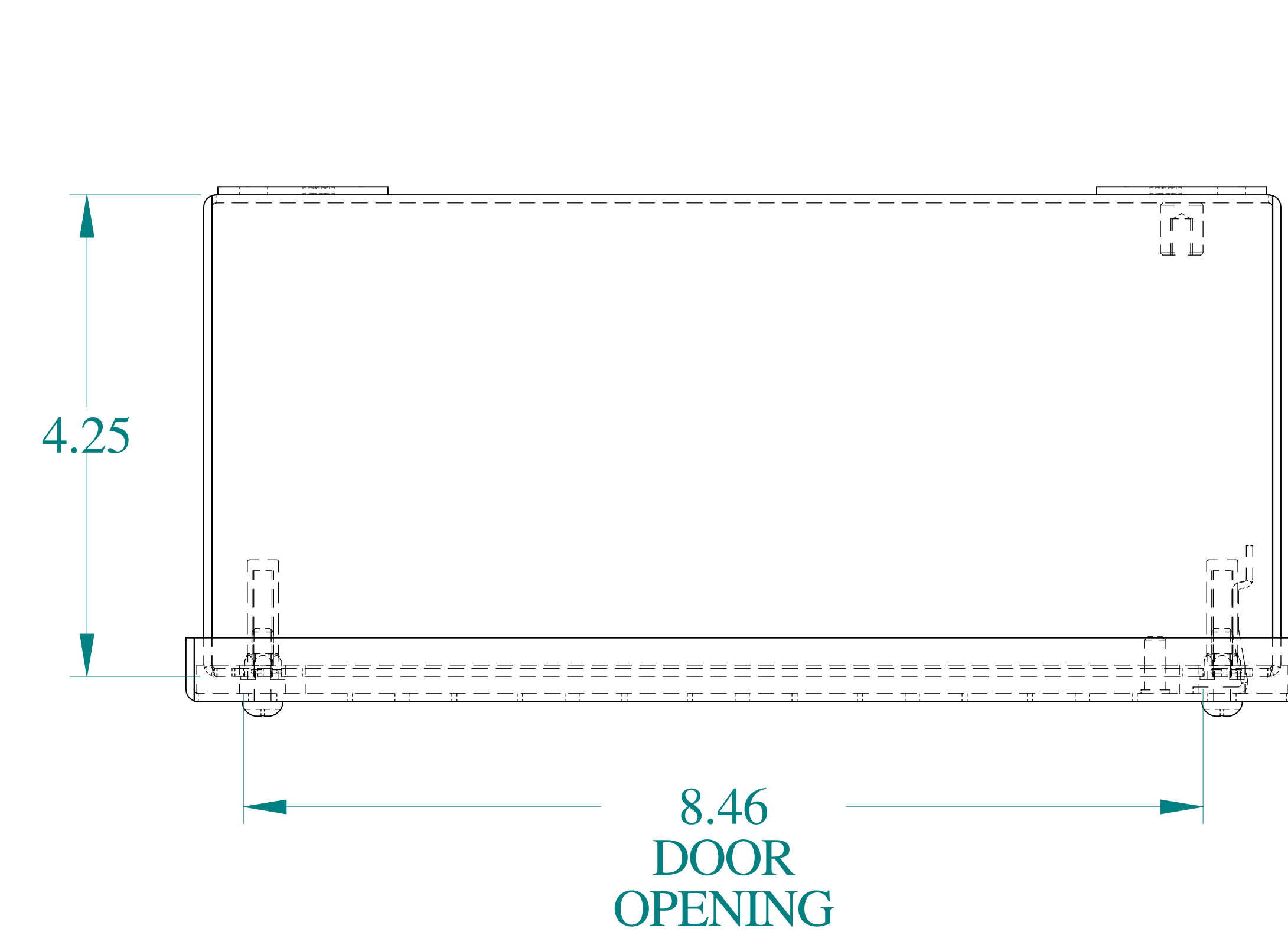
TOP VIEW
