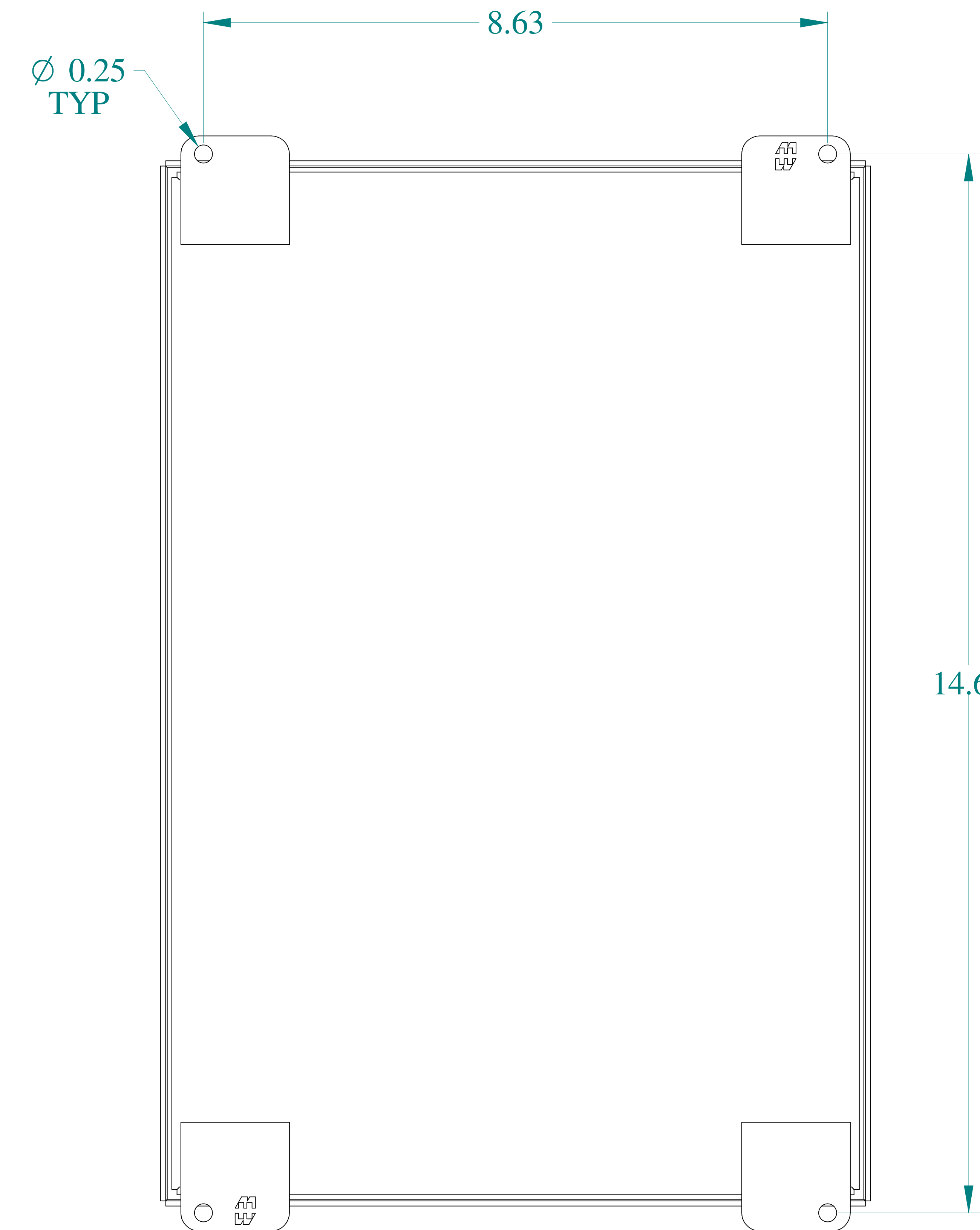
BACK VIEW
