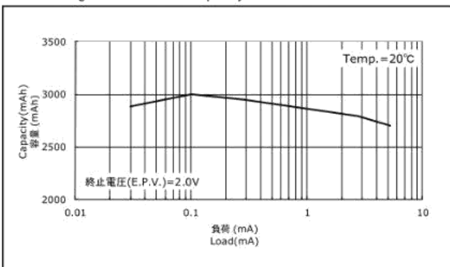
Discharge Load vs. Cell Capacity of CR8·LHC
