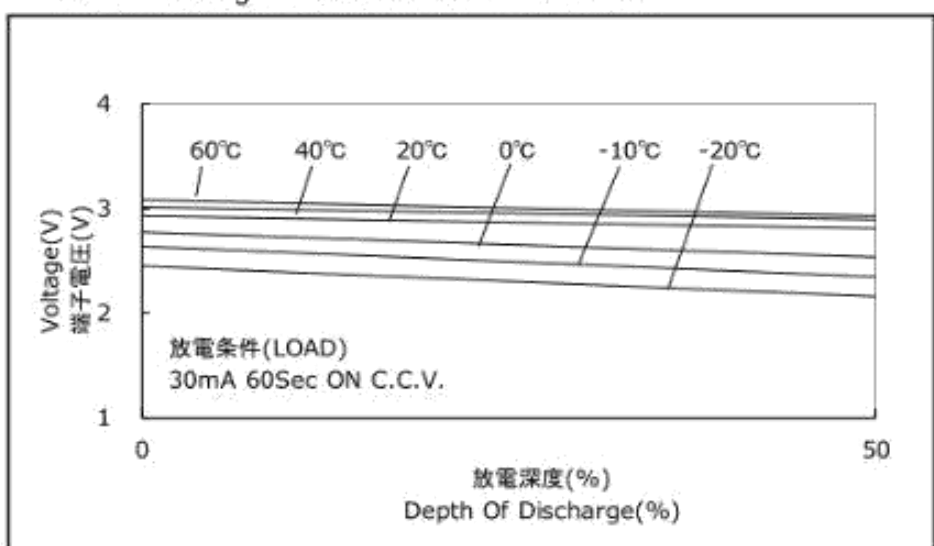
Pulse discharge Characteristics of CR8·LHC
