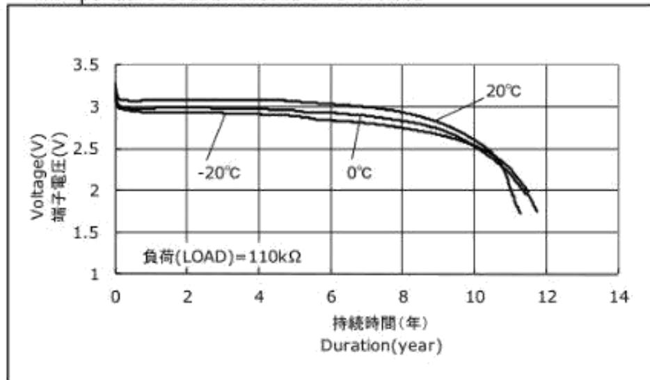
Temperature Characteristics of CR8·LHC
