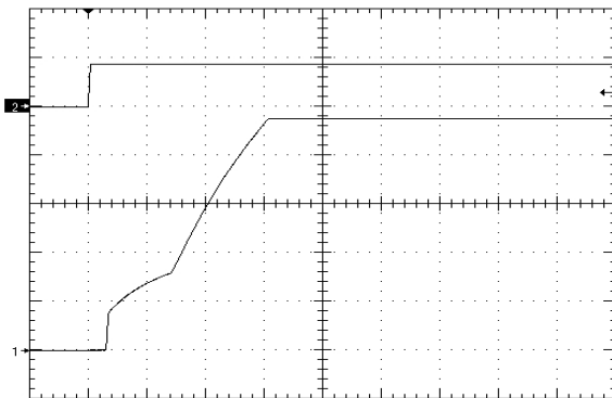
Figure 9. Startup Waveform via Enable Pin, time scale 20mS/div. Vin=Vin_nom, no load Ch1=10V/div, Ch2=5V/div
