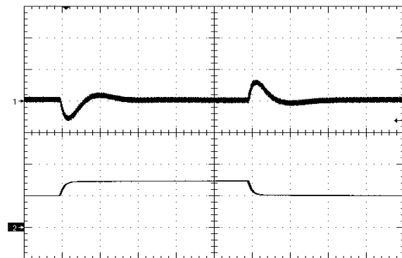
Figure 12. Load Transient Response (100mV/div), di/dt=0.1A/uS, 50% - 75% - 50% of full load +220uF Ch2=1A/div, time scale: 200uS/div
