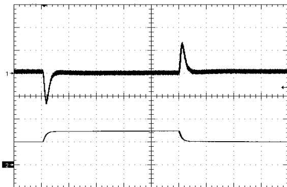
Figure 11. Load Transient Response (100mV/div), di/dt=0.1A/uS, 50% - 75% - 50% of full load, Ch2=1A/div, time scale: 200uS/div
