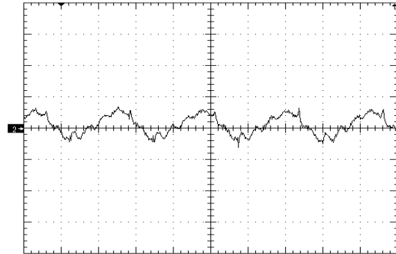
Figure 8. Input Reflected Ripple Current (10mA/div) time scale - 1uS/div. Vin=Vin_nom, full resistive.
