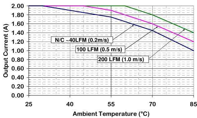
Figure 3. Output Current Derating vs Ambient Temperature & Airflow (air flowing from pin 3 to pin 1, Vin = 48 V, with baseplate)
