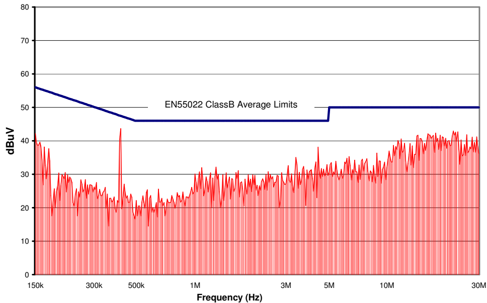
Figure 18. CPE2U36 Conducted Emissions using above specified input filter, Vin = 48V, Full Resistive Load
