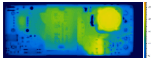
Thermal Image of module @ 48Vin, 200LFM & 55C
