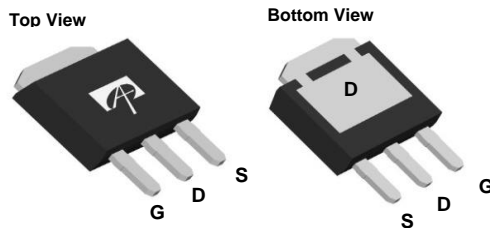
TO251B (IPAK short lead)
