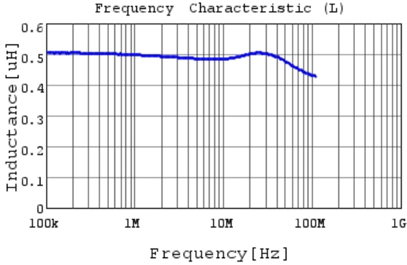
LQM18PHR47MFR L
