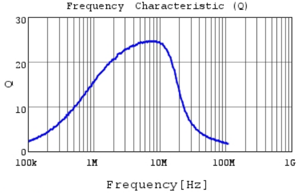
LQM18PHR47MFR Q
