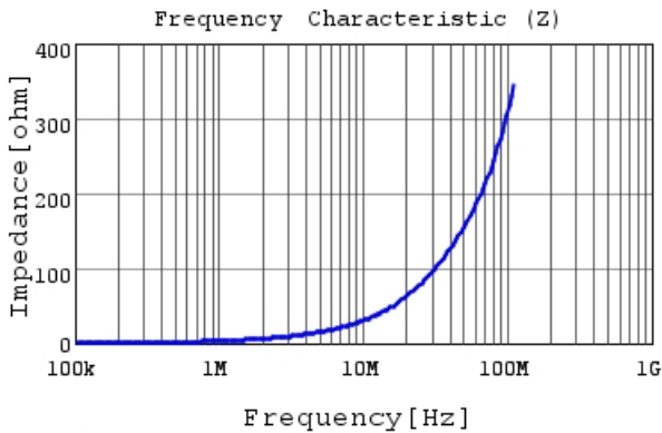
LQM18PHR47MFR |Z|
