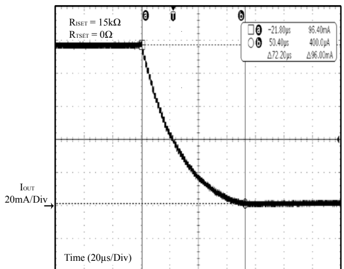
Figure 32 Instant Off
