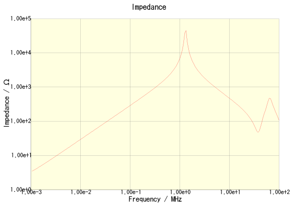
CLF6045T-471M-CA
