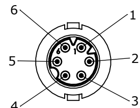
FACE VIEW 16980-6PG-5XX 6 POSITION B-KEY
