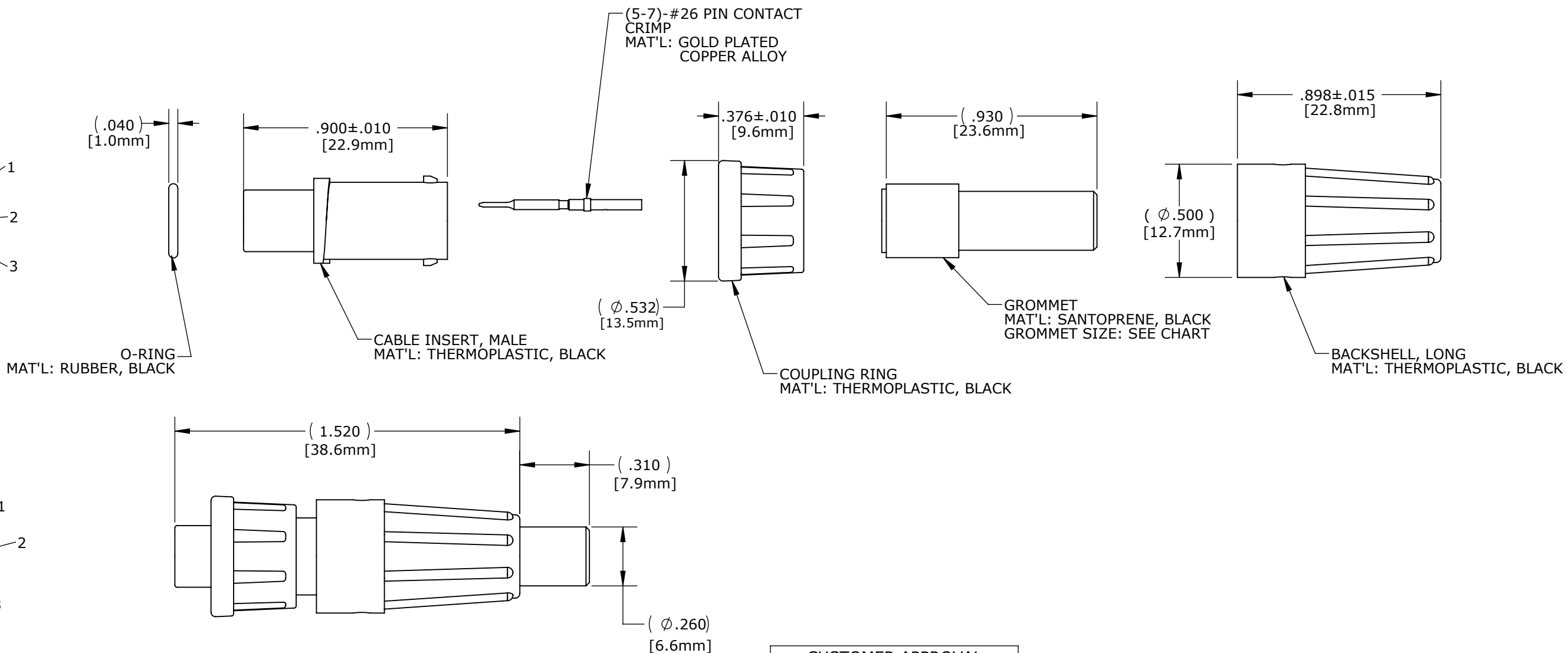
ASSEMBLED KIT VIEW FOR CUSTOMER REFERENCE ONLY
