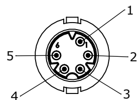
FACE VIEW 16980-5PG-5XX 5 POSITION A-KEY
