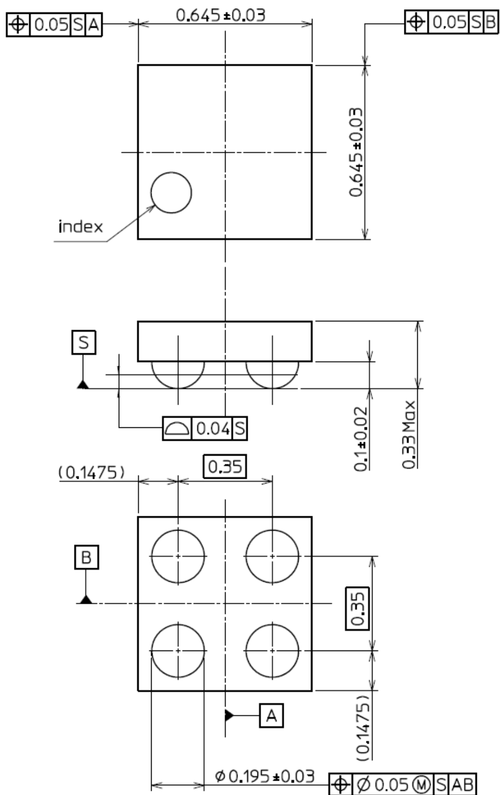
Figure 11.1 Package Dimensions
