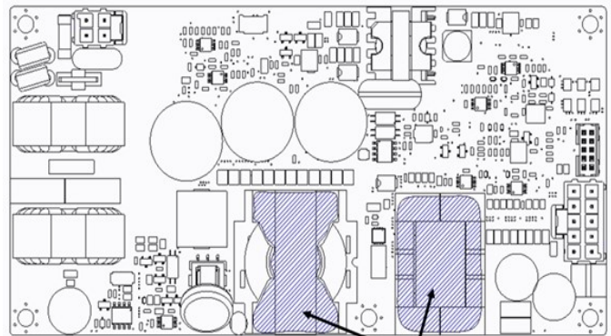
THERMALLY TIED TO TOP OF ENCLOSURE
