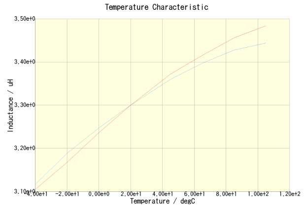
CLF6045T-3R3N-CA(DC = 0A)
