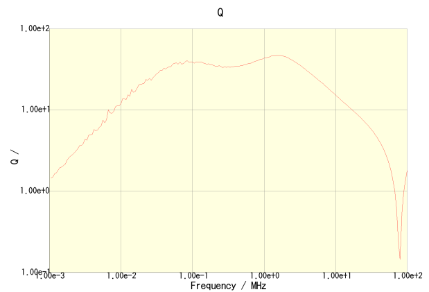
CLF6045T-3R3N-CA
