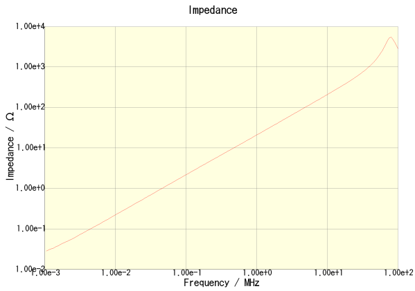
CLF6045T-3R3N-CA
