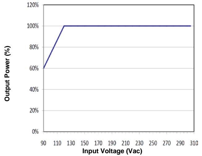
Figure 14: Output Power vs. Input Voltage
