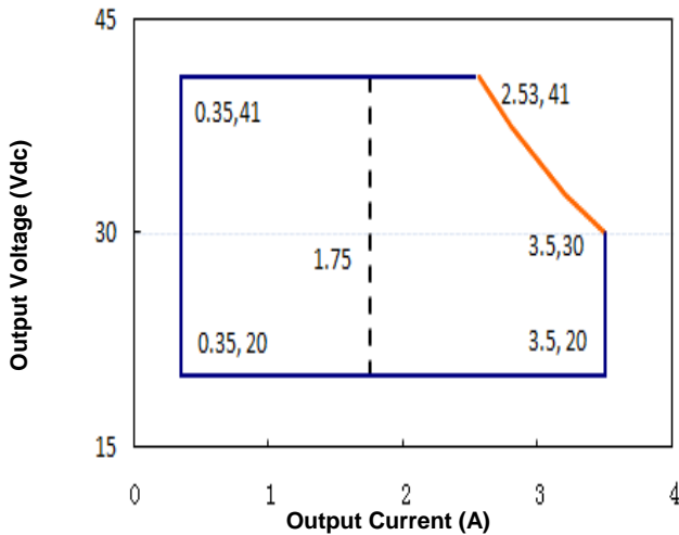
Figure 1: Typical V-I Characteristic Curve (LUB105X-041CP)
