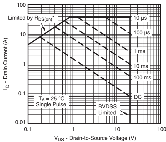
* V_{GS} > \text{minimum } V_{GS} \text{ at which } R_{DS(on)} \text{ is specified} Safe Operating Area, Junction-to-Ambient
