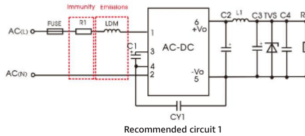
Recommended circuit 1
