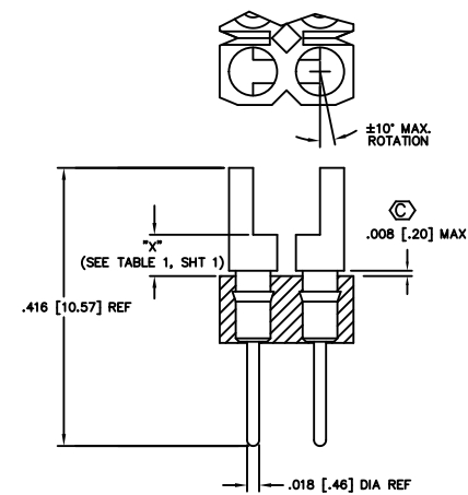
FIG 8 TERMINAL STYLE -C T-1R2-X
