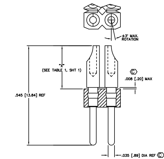
FIG 7 TERMINAL STYLE -B-2 T-1R8-2-X
