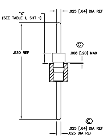
FIG 3 TERMINAL STYLE -A-1 T-1R7-1-X
