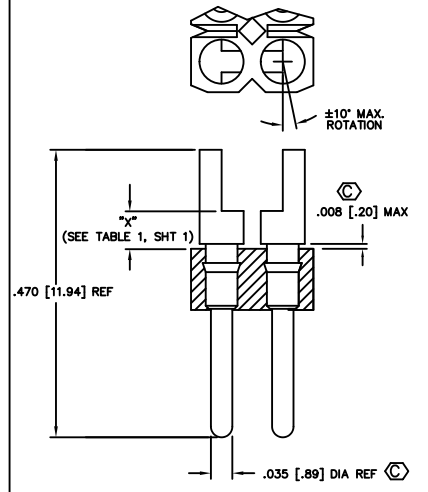
FIG 10 TERMINAL STYLE -C-2 T-1R9-2-X
