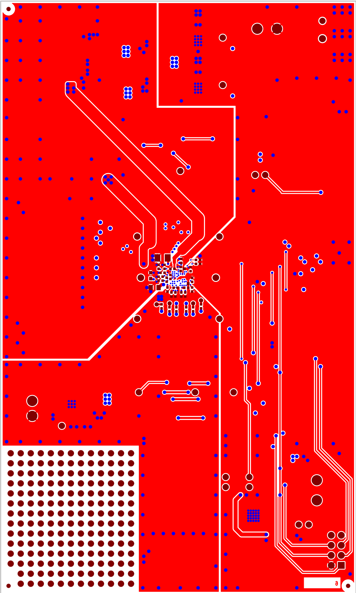
EVAL-ADuCM310EBZ (Rev C) Top Side View
