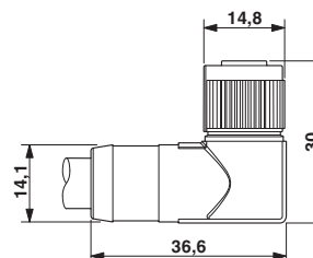
Socket M12-SPEEDCON, angled, shielded
