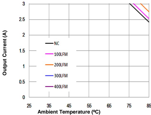
Figure 9. Current Derating Curve with Open Frame (Direction 3 (Ref. Figure 10); typical V_{in} , soldered interface)
