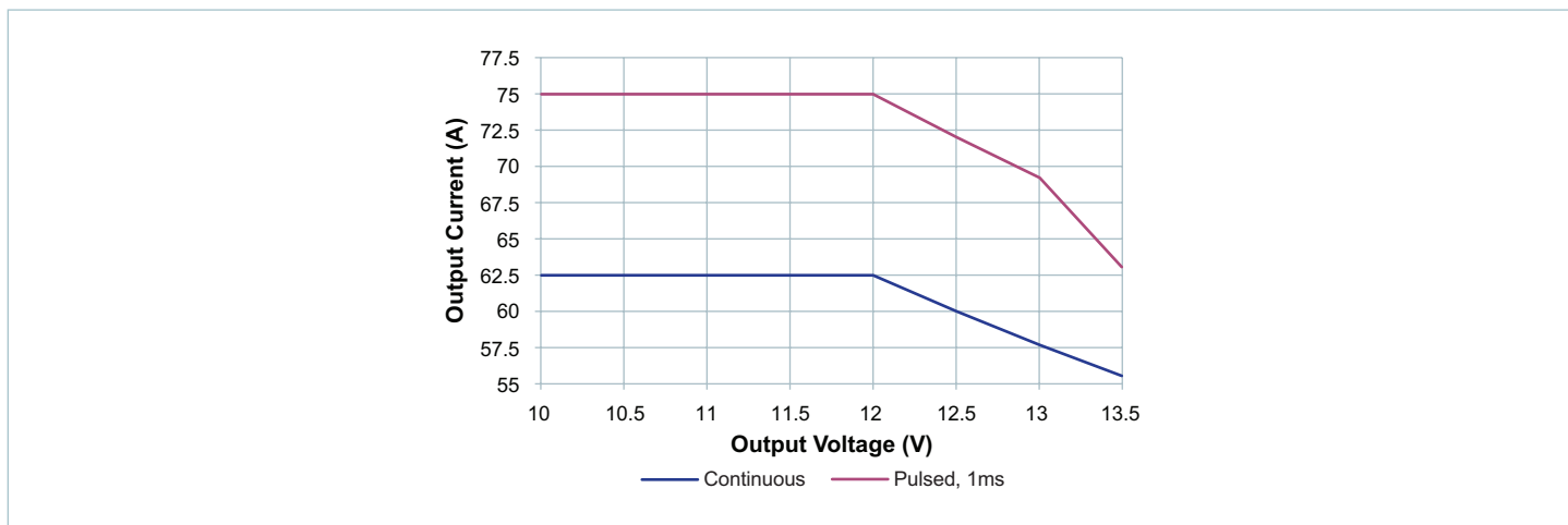
Figure 1 — Electrical specified operating area vs. V_{OUT}
