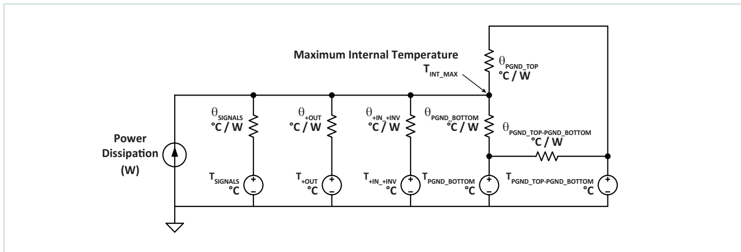
Figure 23 — Thermal model
