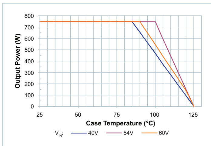
Figure 3 — Thermal specified operating area; double-sided cooling, output power vs. case temperature, nominal trim
