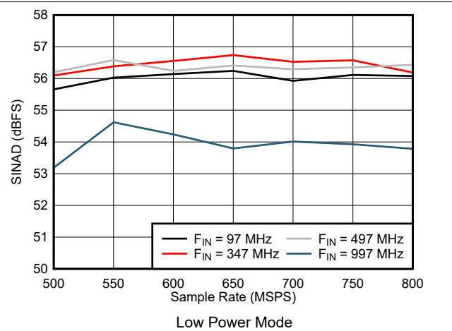
Figure 7-56. SINAD vs Sample Rate in Low Power Mode
