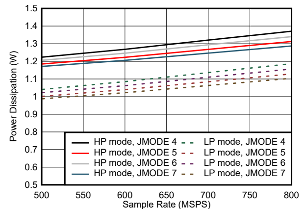
Figure 7-89. Dual Channel, Power Dissipation vs F_S for JMODES 4 - 7
