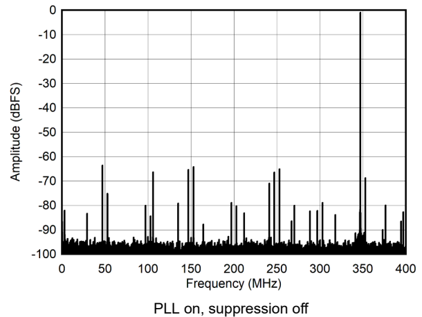
Figure 7-14. Single Tone FFT at 347 MHz and -1dBFS
