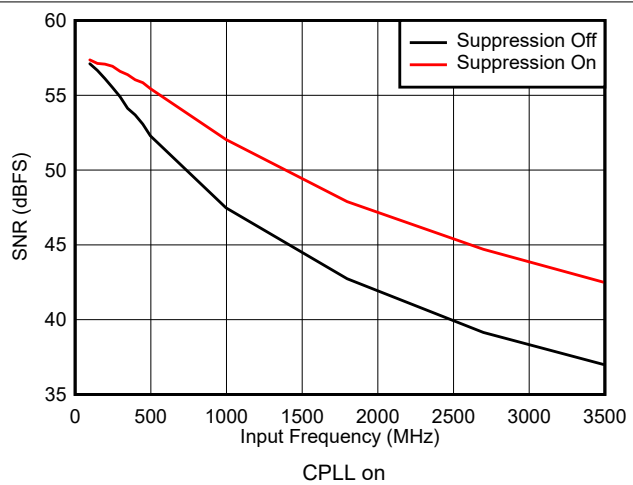
Figure 7-34. SNR vs Input Frequency and Suppression
