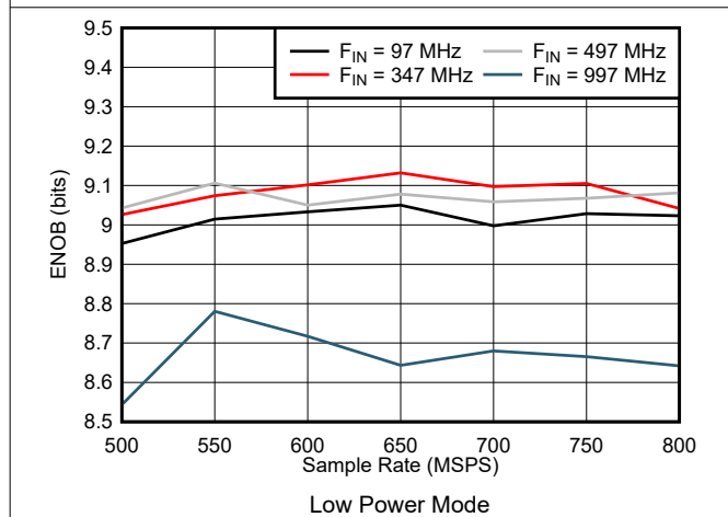
Figure 7-57. ENOB vs Sample Rate in Low Power Mode
