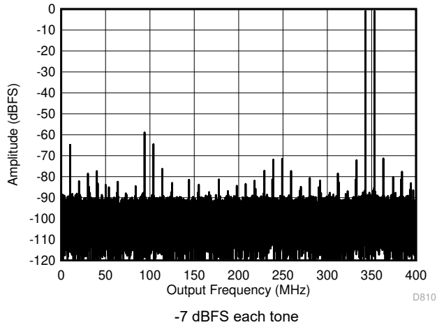
Figure 7-69. Two Tone FFT at 347 MHz in Low Power Mode
