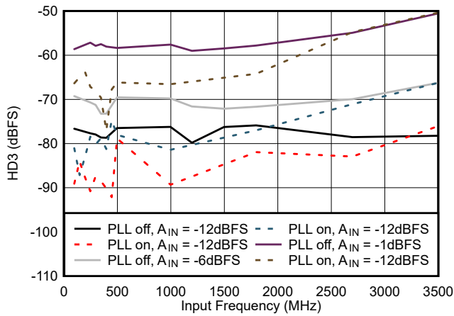
Figure 7-25. HD3 vs Input Frequency
