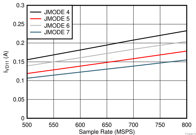
Figure 7-95. Dual Channel, I_{VD11} vs F_S for JMODES 4 - 7
