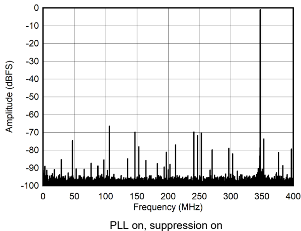
Figure 7-15. Single Tone FFT at 347 MHz and -1dBFS
