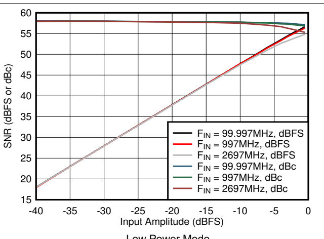
Figure 7-58. SNR vs Input Amplitude in Low Power Mode
