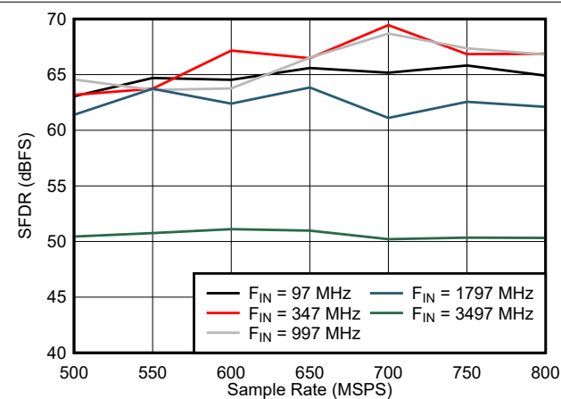
Figure 7-29. SFDR vs Sample Rate
