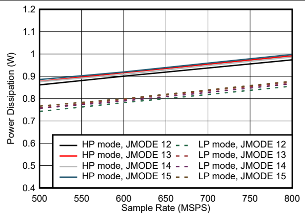
Figure 7-104. Single Channel, Power Dissipation vs F_S for JMODES 12 - 15
