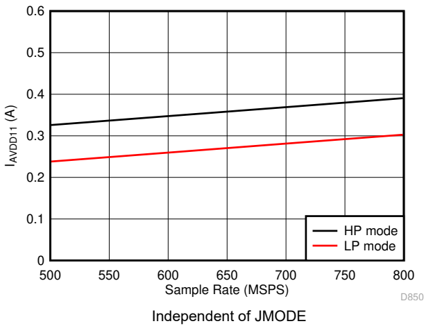
Independent of JMODE Figure 7-93. Dual Channel, I_{VA11} vs F_S
