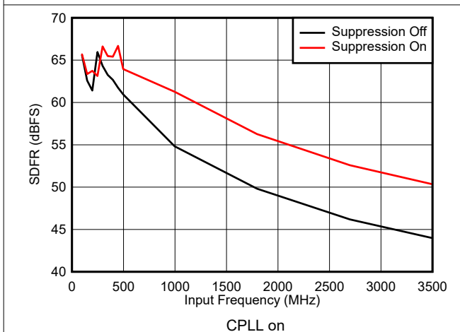
Figure 7-35. SFDR vs Input Frequency and Suppression
