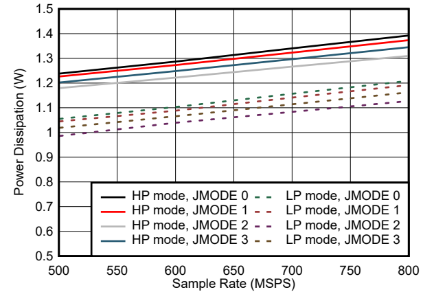
Figure 7-88. Dual Channel, Power Dissipation vs F_S for JMODES 0 - 3
