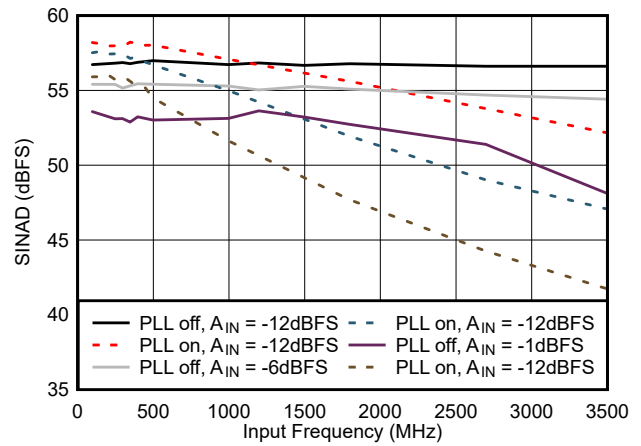
Figure 7-26. SINAD vs Input Frequency
