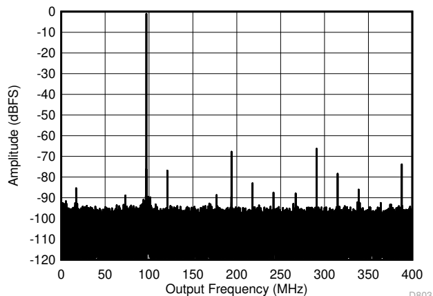
Figure 7-7. Single Tone FFT at 897 MHz and -1dBFS
