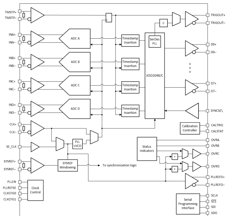
Quad Channel Block Diagram
