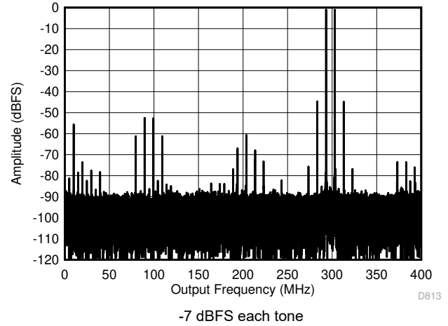
Figure 7-68. Two Tone FFT at 3498 MHz
