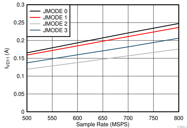
Figure 7-94. Dual Channel, I_{VD11} vs F_S for JMODES 0 - 3
