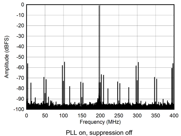
Figure 7-16. Single Tone FFT at 997 MHz and -1dBFS
