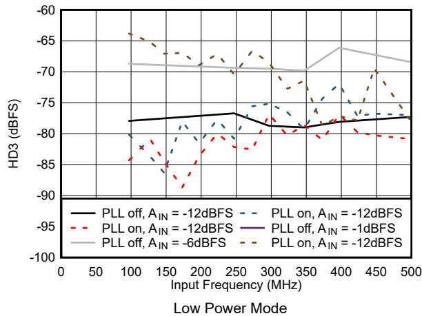
Figure 7-51. HD3 vs Input Frequency in Low Power Mode
