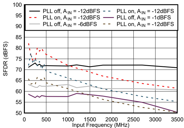
Figure 7-23. SFDR vs Input Frequency
