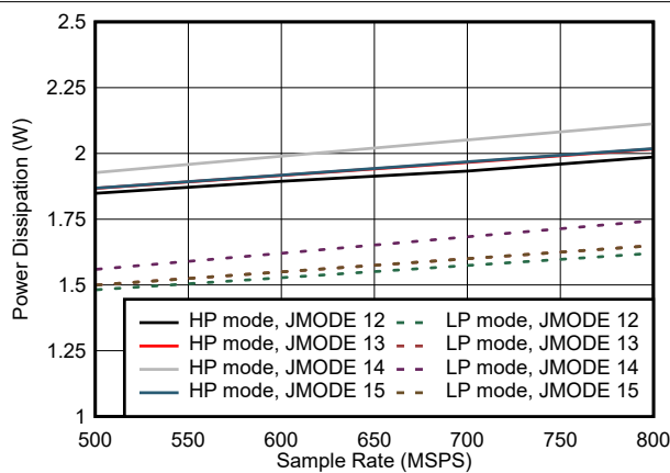
Figure 7-77. Quad Channel, Power Dissipation vs F_S for JMODES 12 - 15
