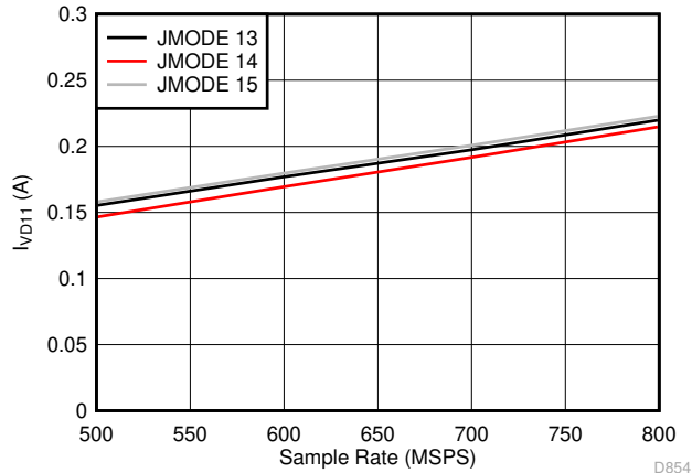
Figure 7-97. Dual Channel, I_{VD11} vs F_S for JMODES 13 - 15
