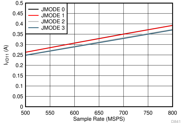
Independent of Power Mode Figure 7-80. Quad Channel, I_{VDD11} vs F_S for JMODES 0 - 3
