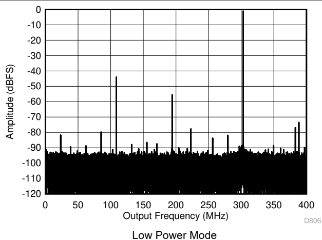
Figure 7-12. Single Tone FFT at 2097 MHz and -1dBFS
