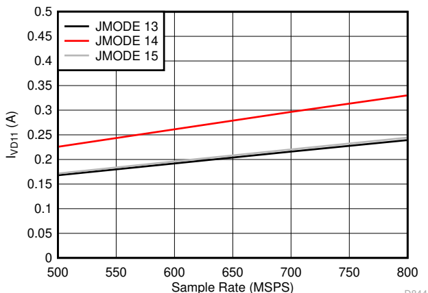
Independent of Power Mode Figure 7-83. Quad Channel, I_{VDD11} vs F_S for JMODES 13-15
