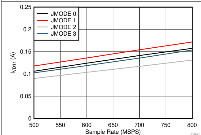
Figure 7-107. Single Channel, I_{VD11} vs F_S for JMODES 0 - 3
