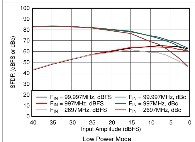
Figure 7-59. SFDR vs Input Amplitude in Low Power Mode
