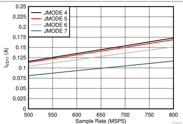
Figure 7-108. Single Channel, I_{VD11} vs F_S for JMODES 4 - 7
