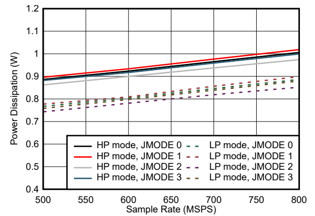
Figure 7-101. Dual Channel, Power Dissipation vs F_S for JMODES 0 - 3
