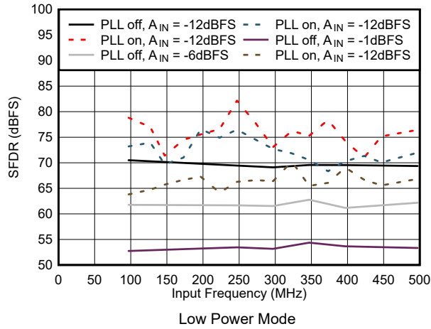
Figure 7-49. SFDR vs Input Frequency in Low Power Mode
