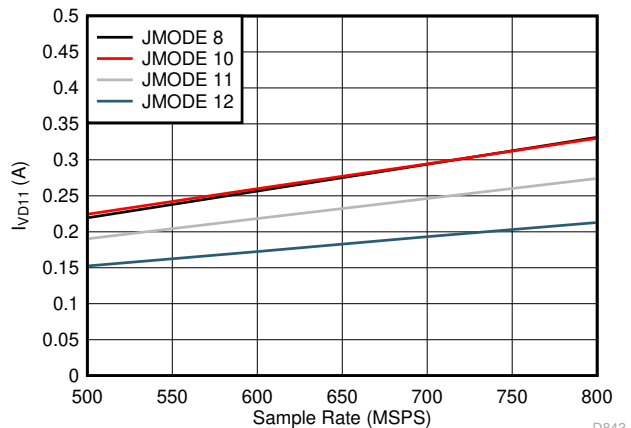
Independent of Power Mode Figure 7-82. Quad Channel, I_{VDD11} vs F_S for JMODES 8-12
