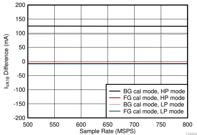
Figure 7-99. Dual Channel, I_{VA19} vs F_S over Modes
