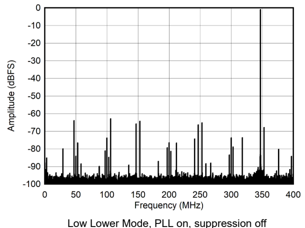
Figure 7-18. Single Tone FFT at 347 MHz and -1dBFS
