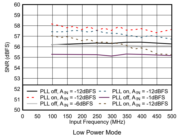
Figure 7-48. SNR vs Input Frequency in Low Power Mode
