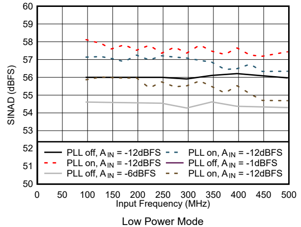
Figure 7-52. SINAD vs Input Frequency in Low Power Mode
