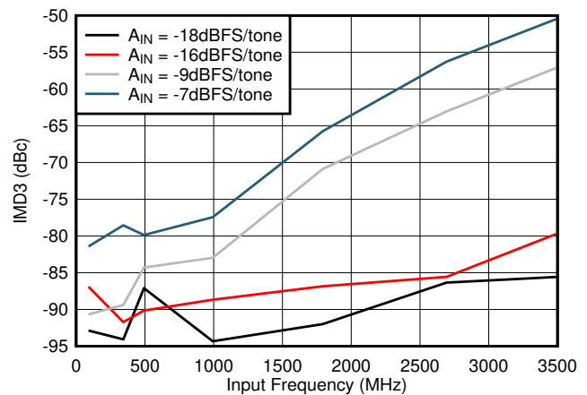
Figure 7-72. IMD3 vs Input Frequency
