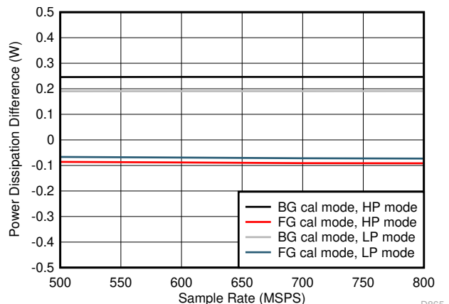
Difference to LPBG mode Figure 7-84. Quad Channel, Power Dissipation vs F_S over Modes
