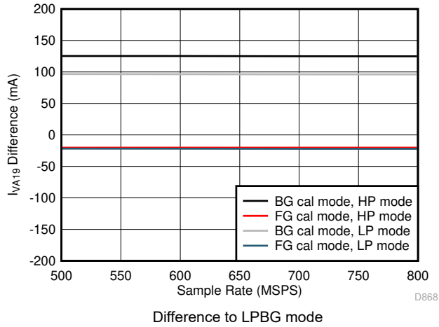
Figure 7-85. Quad Channel, I_{VA19} vs F_S over Modes
