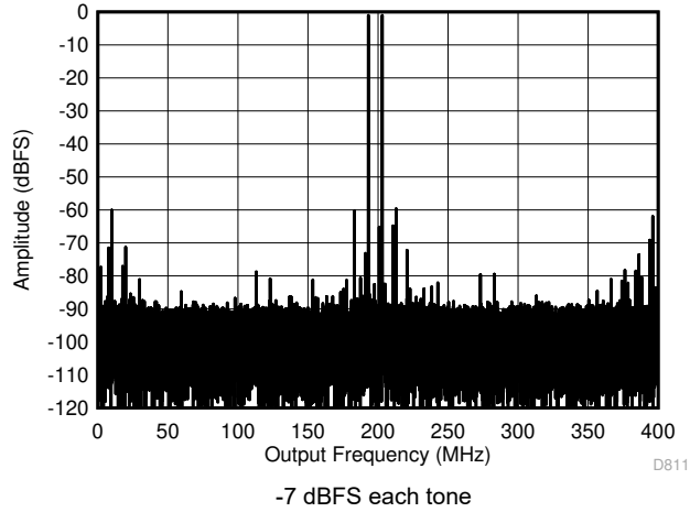
Figure 7-67. Two Tone FFT at 1798 MHz
