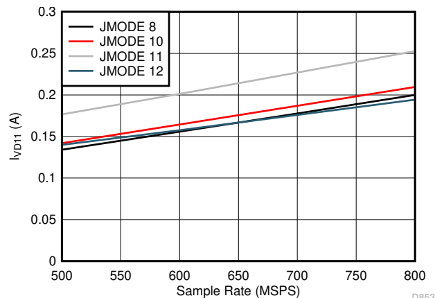
Figure 7-96. Dual Channel, I_{VD11} vs F_S for JMODES 8 - 12
