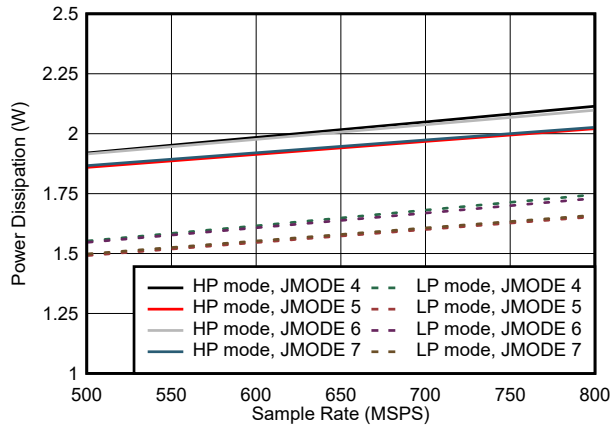
Figure 7-75. Quad Channel, Power Dissipation vs F_S for JMODES 4 - 7
