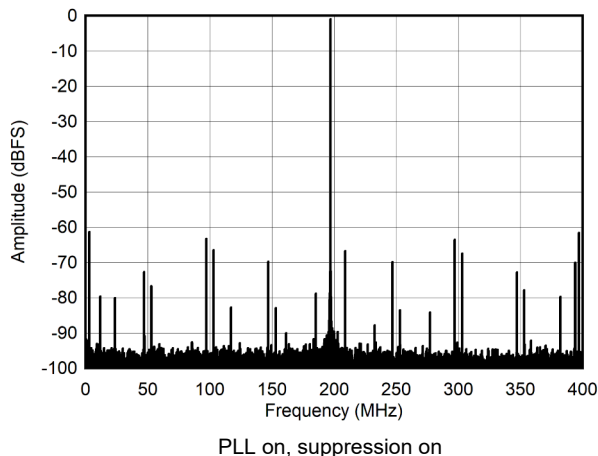
Figure 7-17. Single Tone FFT at 997 MHz and -1dBFS
