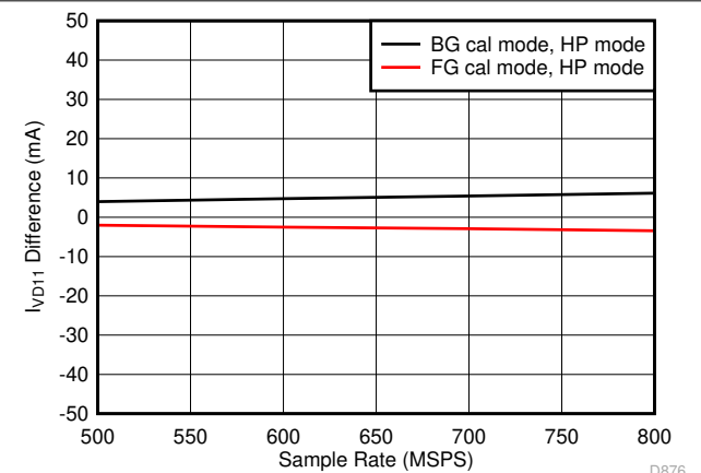
Figure 7-114. Single Channel, I_{VD11} vs F_S over Modes
