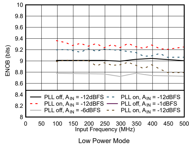
Figure 7-53. ENOB vs Input Frequency in Low Power Mode
