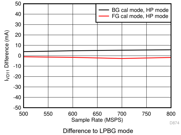
Figure 7-87. Quad Channel, I_{VD11} vs F_S over Modes
