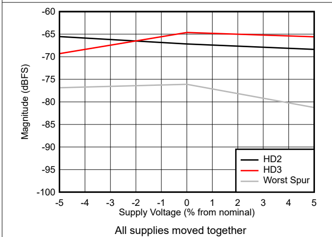
Figure 7-39. HD2, HD3 and worst non-HD vs Supply Voltage
