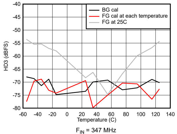
Figure 7-46. HD3 vs Temperature
