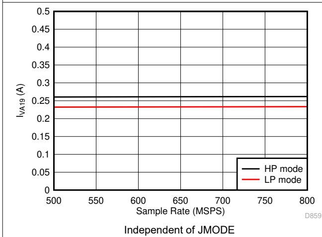
Figure 7-105. Single Channel, I_{VA19} vs F_S
