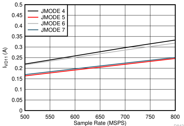
Independent of Power Mode Figure 7-81. Quad Channel, I_{VDD11} vs F_S for JMODES 4 - 7
