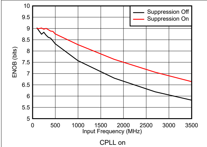
Figure 7-37. ENOB vs Input Frequency and Suppression
