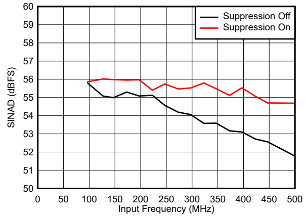
Figure 7-62. SINAD vs Input Frequency
