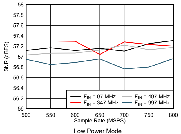
Figure 7-54. SNR vs Sample Rate in Low Power Mode
