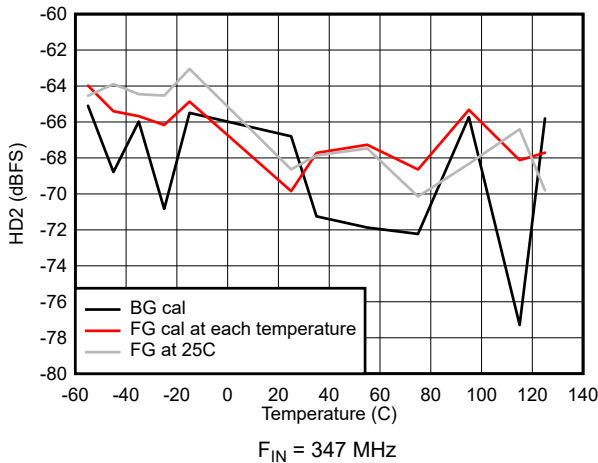
Figure 7-45. HD2 vs Temperature
