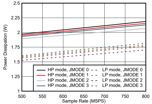
Figure 7-74. Quad Channel, Power Dissipation vs F_S for JMODES 0 - 3
