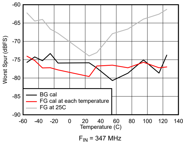
Figure 7-47. worst non-HD spur vs Temperature
