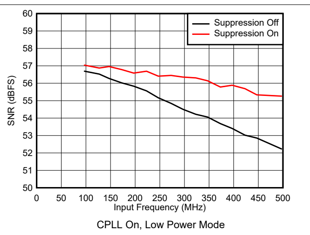
Figure 7-60. SNR vs Input Frequency
