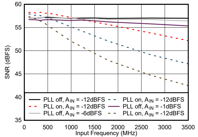
Figure 7-22. SNR vs Input Frequency
