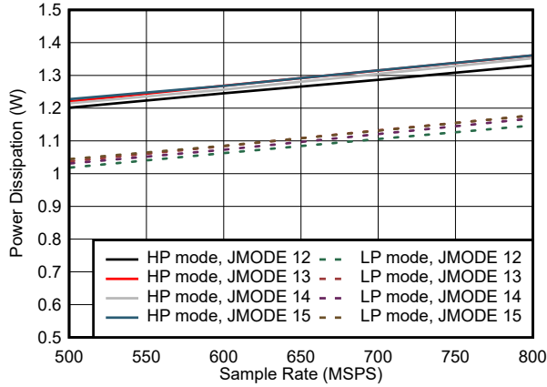
Figure 7-91. Dual Channel, Power Dissipation vs F_S for JMODES 12 - 15
