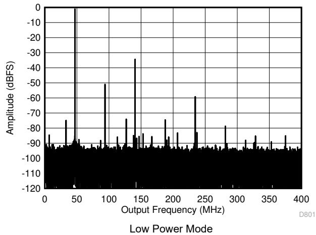
Figure 7-13. Single Tone FFT at 3247 MHz and -1dBFS
