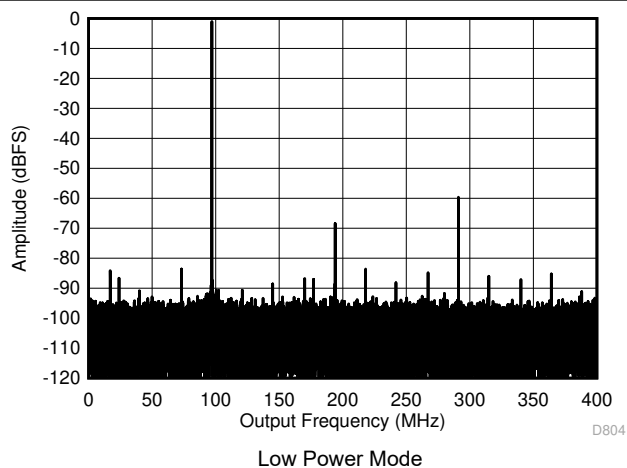
Figure 7-11. Single Tone FFT at 897 MHz and -1dBFS
