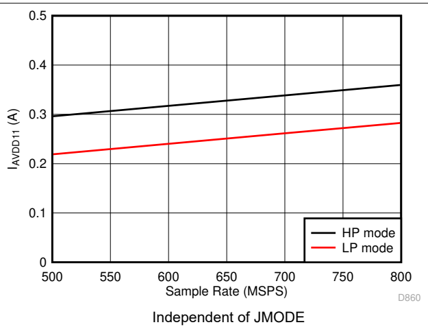
Figure 7-106. Single Channel, I_{VA11} vs F_S
