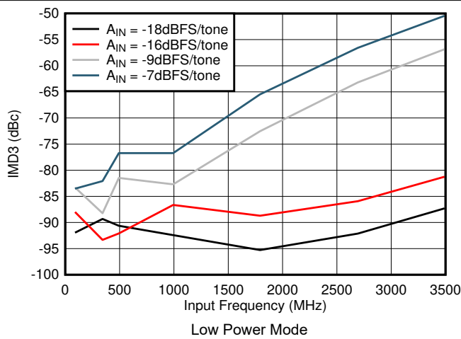
Figure 7-73. IMD3 vs Input Frequency in Low Power Mode
