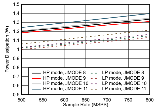
Figure 7-90. Dual Channel, Power Dissipation vs F_S for JMODES 8 - 11
