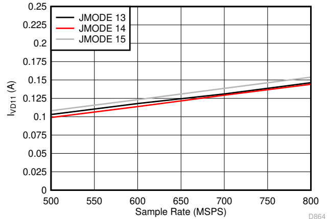
Figure 7-110. Single Channel, I_{VD11} vs F_S for JMODES 13 - 15
