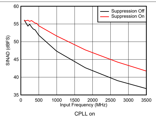
Figure 7-36. SINAD vs Input Frequency and Suppression
