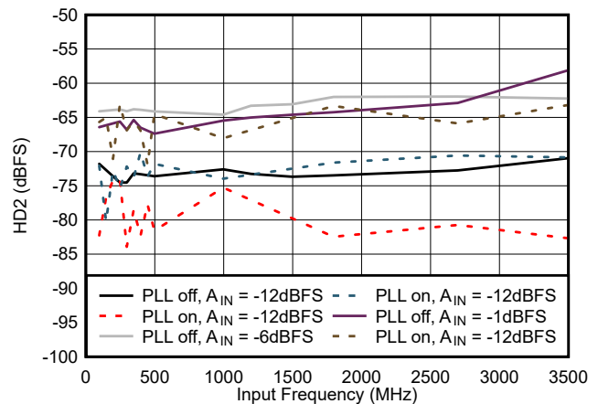
Figure 7-24. HD2 vs Input Frequency
