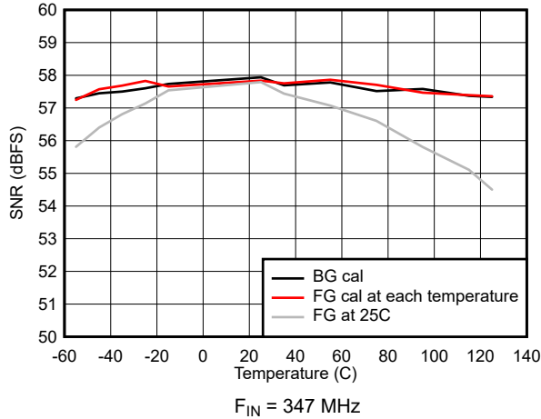
Figure 7-43. SNR vs Temperature
