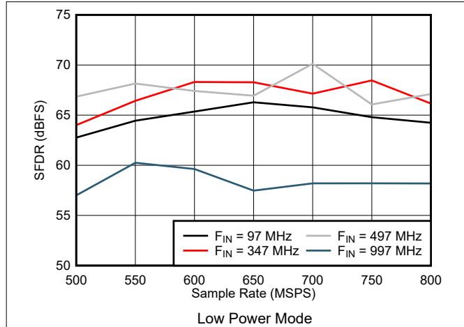
Figure 7-55. SFDR vs Sample Rate in Low Power Mode
