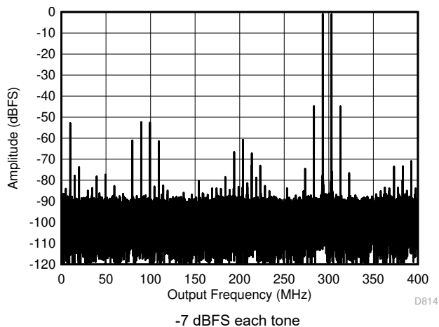
Figure 7-71. Two Tone FFT at 3498 MHz in Low Power Mode
