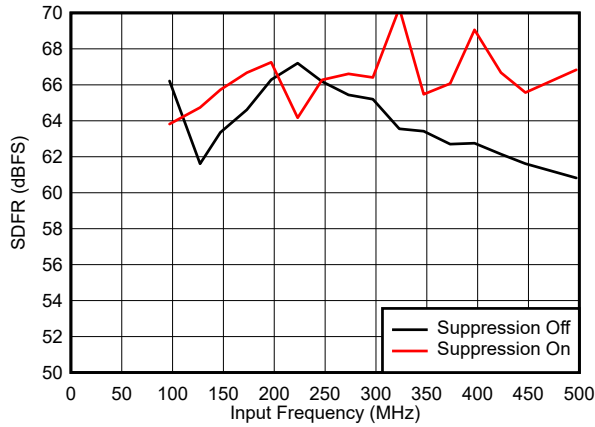
Figure 7-61. SFDR vs Input Frequency
