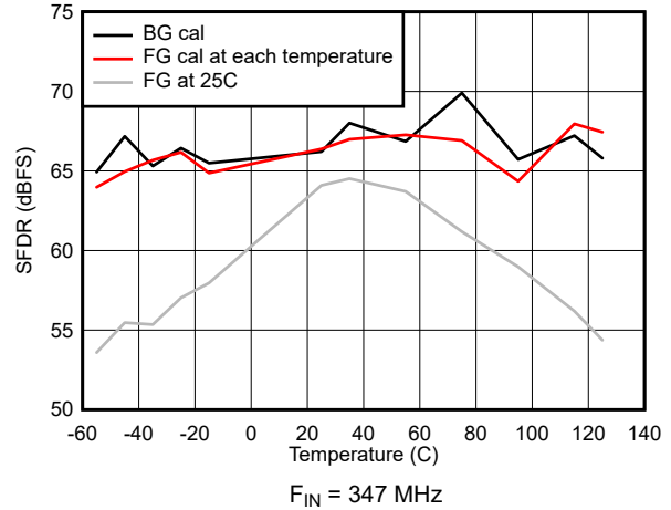
Figure 7-44. SFDR vs Temperature
