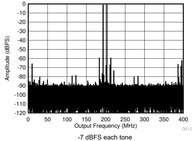
Figure 7-70. Two Tone FFT at 1798 MHz in Low Power Mode
