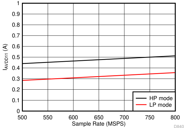
Independent of JMODE Figure 7-79. Quad Channel, I_{VDD11} vs F_S
