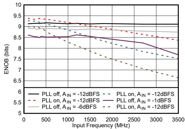
Figure 7-27. ENOB vs Input Frequency
