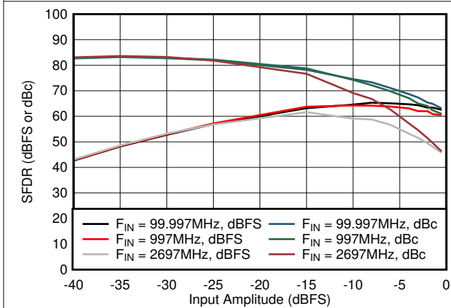
Figure 7-33. SFDR vs Input Amplitude
