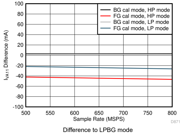
Figure 7-86. Quad Channel, I_{VA11} vs F_S over Modes
