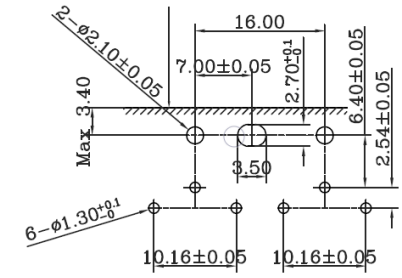
Recommended Mounting Layout
