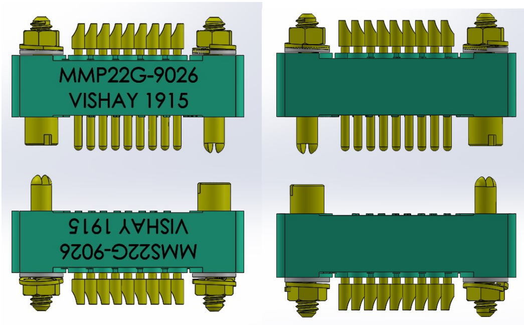
Figure #1: MM Mating Configuration
