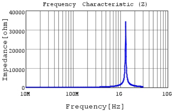
LQG15WZR10G02 |Z|
