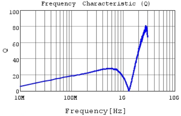
LQG15WZR10G02 Q
