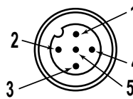
Euro-style Male Pinouts
