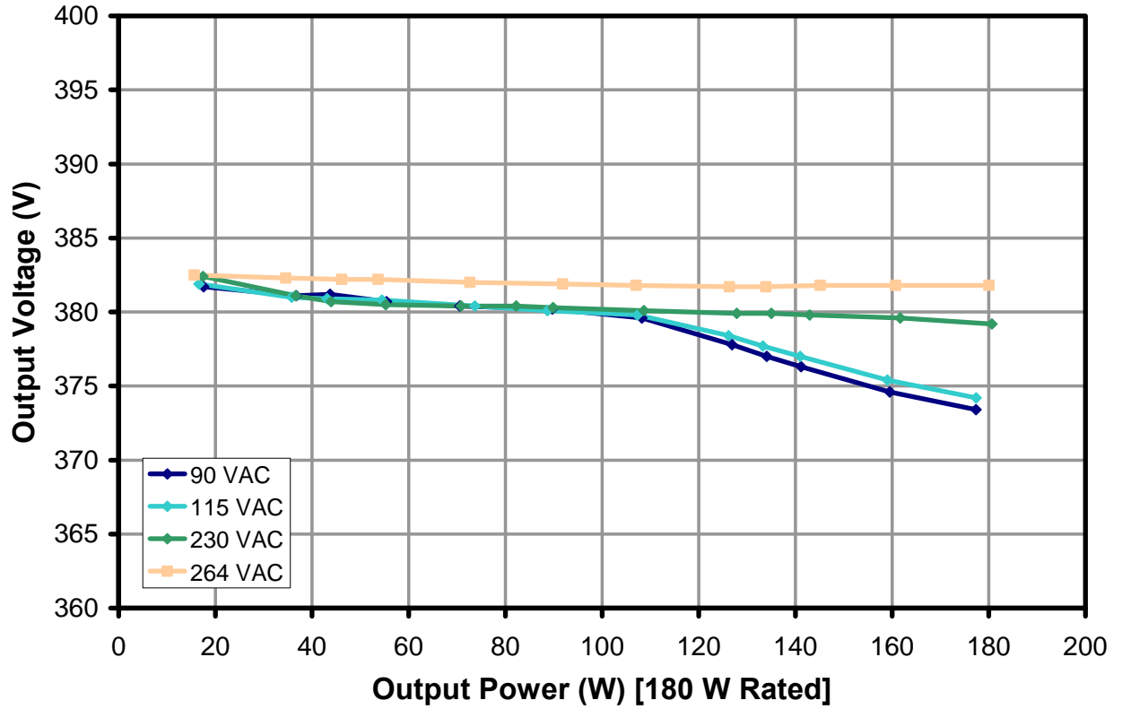
Figure 17 – Load Regulation.
