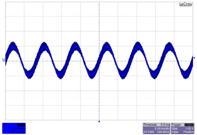
Figure 69 – Ripple, 90 VAC, 100% Load. 5 ms, 5 V / div.
