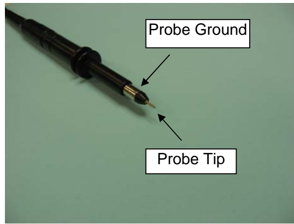
Figure 66 – Oscilloscope Probe Prepared for Ripple Measurement (End Cap and Ground Lead Removed).
