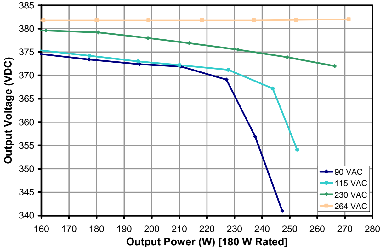
Figure 19 – Overload Regulation.
