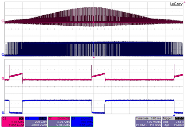
Figure 65 – Input Voltage 230 VAC, 100% Load. Upper: I_{DRAIN} , 2 A / div. Lower: V_{DRAIN} , 200 V / div., 1 ms / div. Zoom Upper: I_{DRAIN} , 2 A / div., Zoom Lower: V_{DRAIN} , 200 V / div., 5 \mu s / div.
