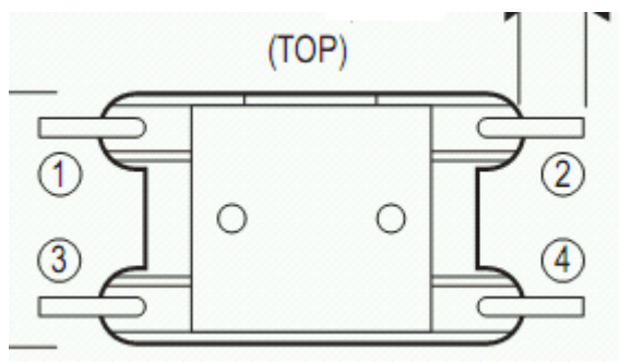
Figure 9 – Top View of Toroid Mounting Base Item [3].
