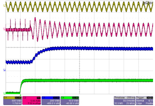
Figure 34 – 115 VAC, Full Load. Upper: V_{IN} , 500 V / div. Second: I_{IN} , 5 A / div. Third: V_{OUT} , 200 V / div. Lower: V_{CC} , 10 V, 50 ms / div.
