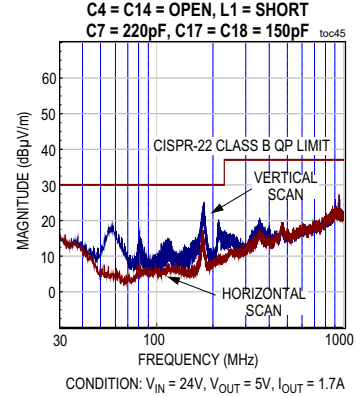
RADIATED EMISSION PLOT
