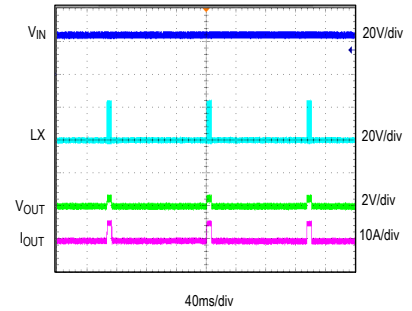
OUTPUT SHORT IN STEADY STATE VIN = 24V, VOUT = 3.3V, IOUT = 0A to SHORT MODE = SGND
