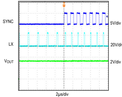
SYNC FREQUENCY AT 740KHZ VIN = 24V, VOUT = 5V, IOUT = 0A, MODE = GND
