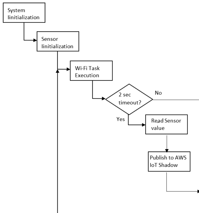
Figure 1-6. Functional Flow
