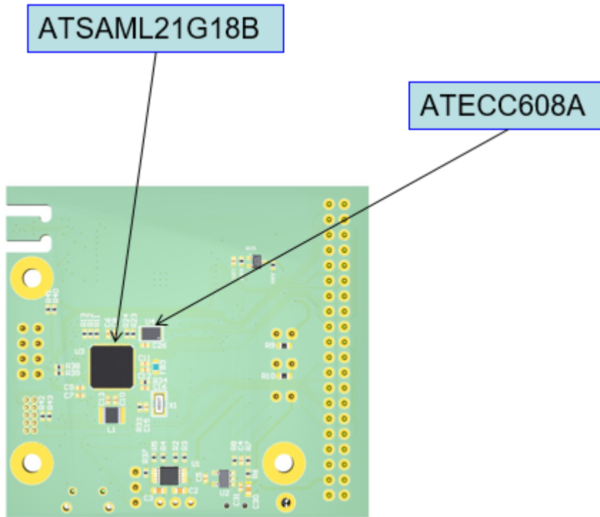
Figure 1-3. Bottom Side
