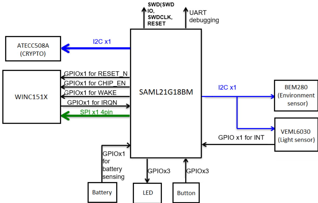
Figure 1-1. Block Diagram
