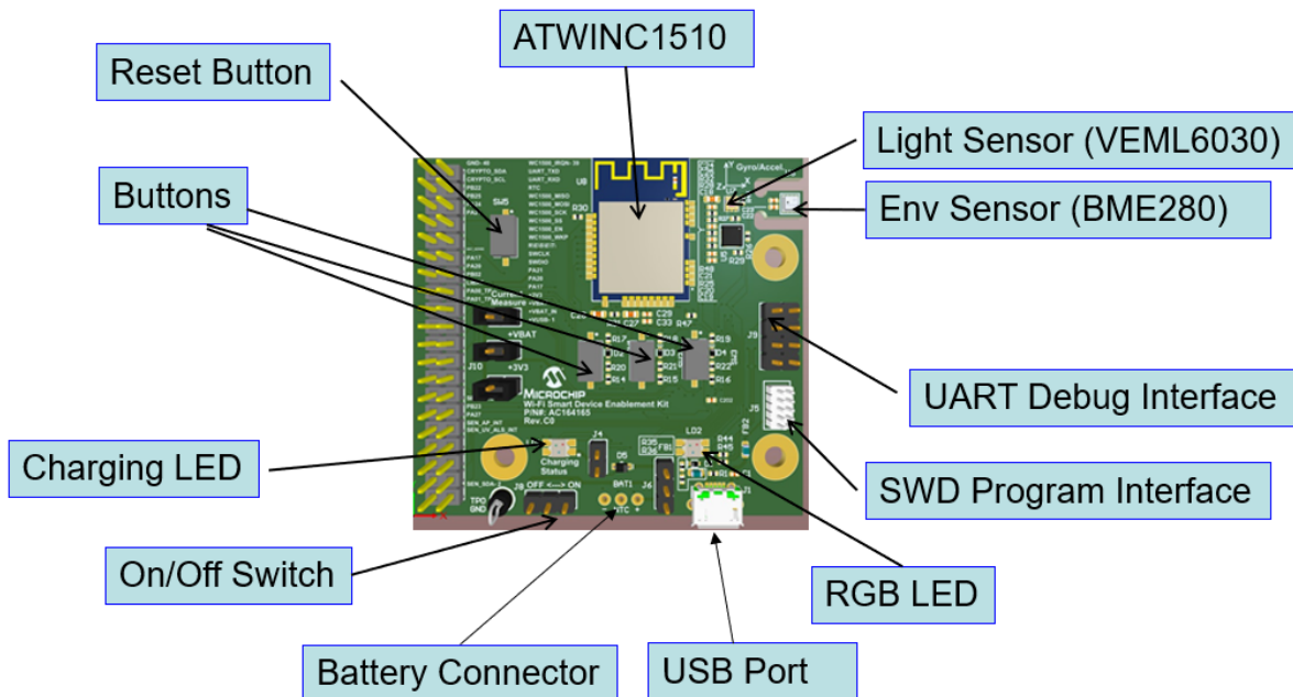
Figure 1-2. Top Side
