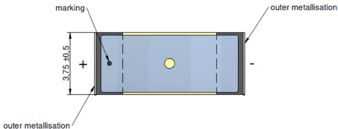
Fig. 1: Dimensional Drawing
