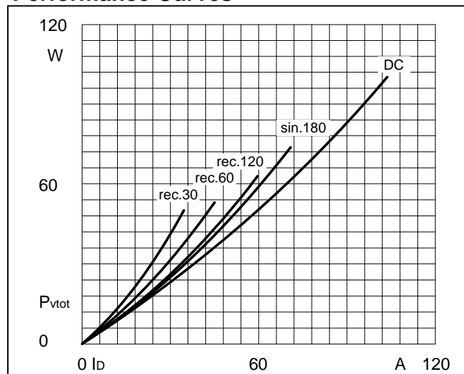
Fig1. Power dissipation
