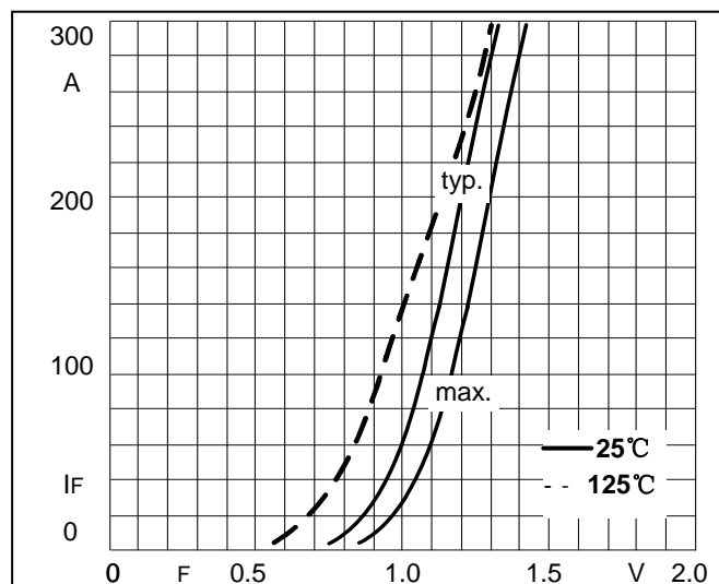
Fig5. Forward Characteristics
