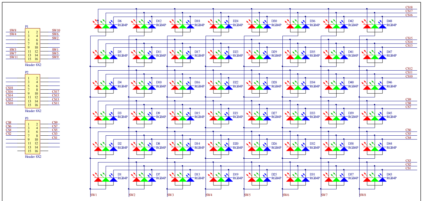
Figure 4: FxLED_6x8_ARRAY Schematic
