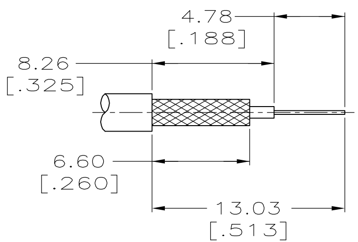
RECOMMENDED STRIP LENGTH SCALE 4:1
